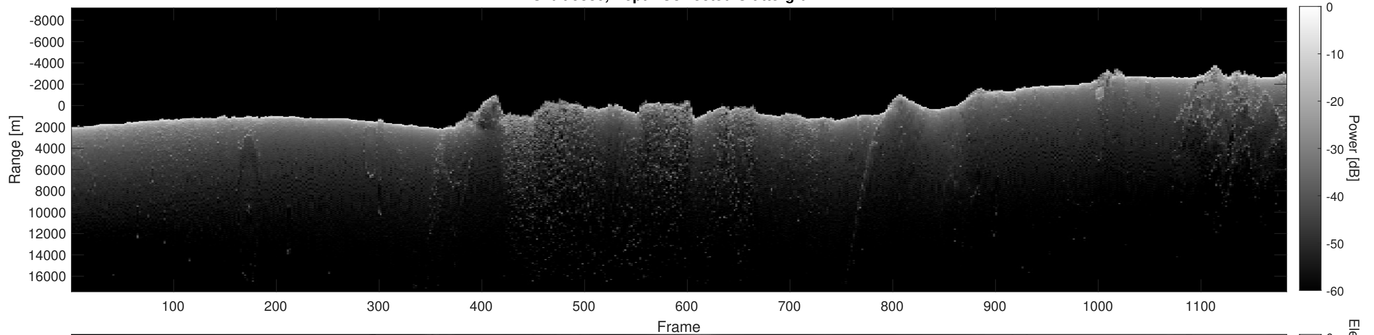
Orbit 9380, Depth-Corrected Cluttergram
