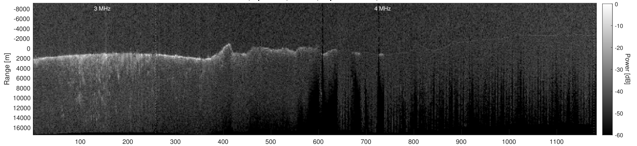
Orbit 9380, Depth-Corrected Cluttergram
