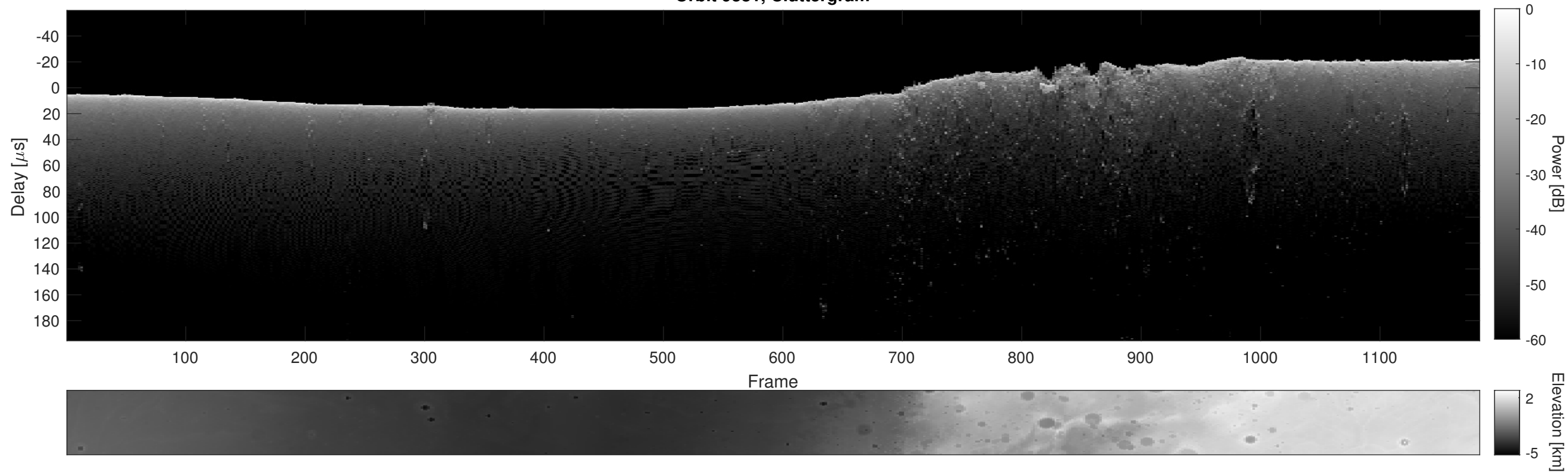
Orbit 9381, Cluttergram
