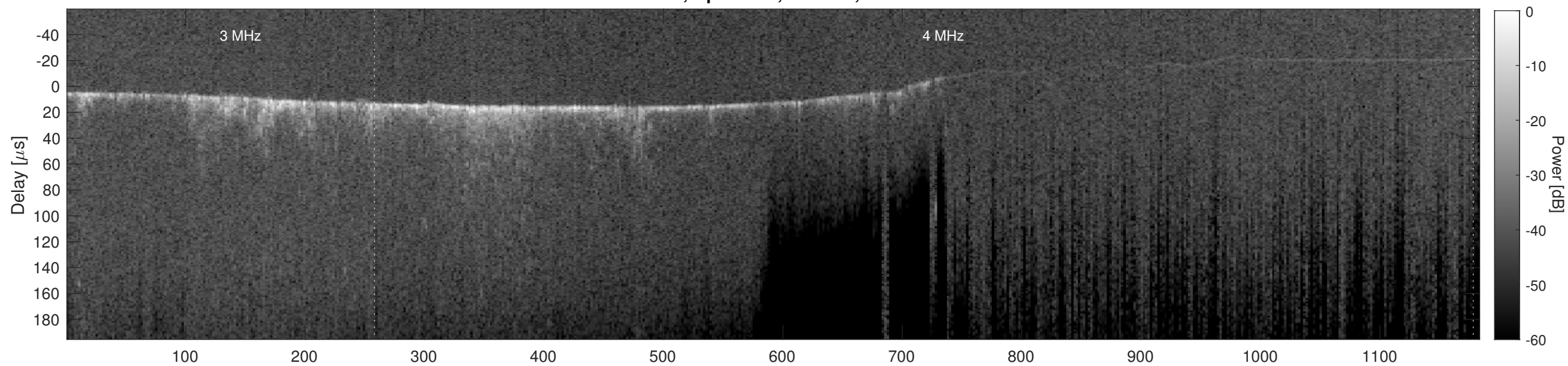
Orbit 9381, Cluttergram
