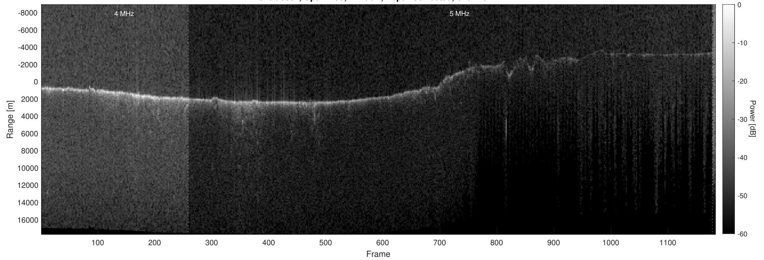
Orbit 9381, Optimized, Window, Depth-Corrected, Channel 2
