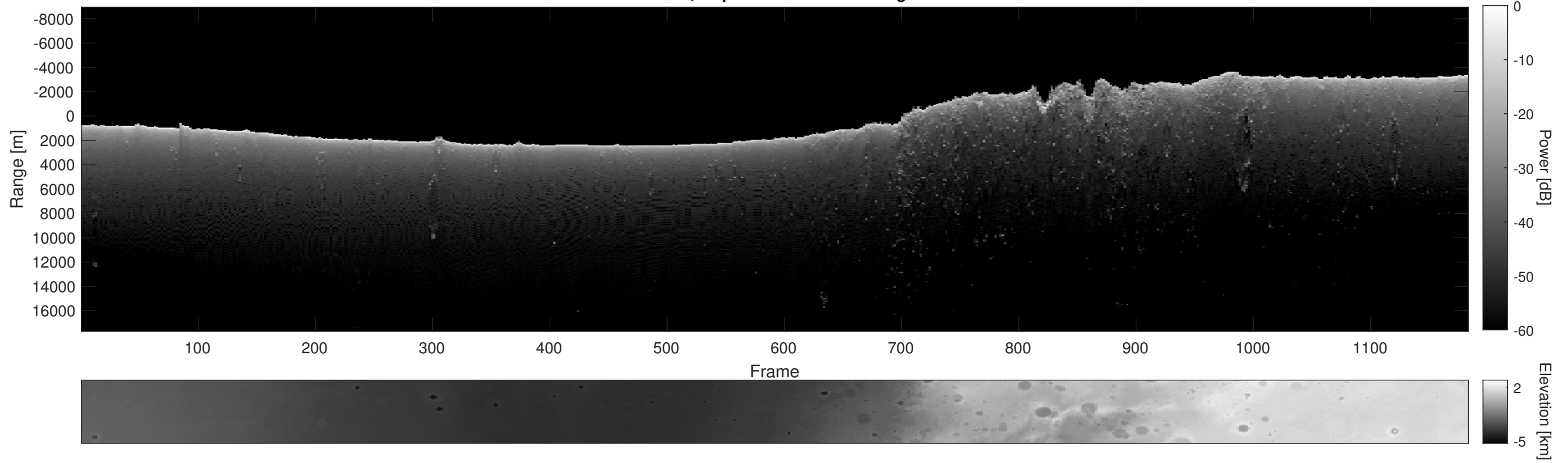
Orbit 9381, Depth-Corrected Cluttergram
