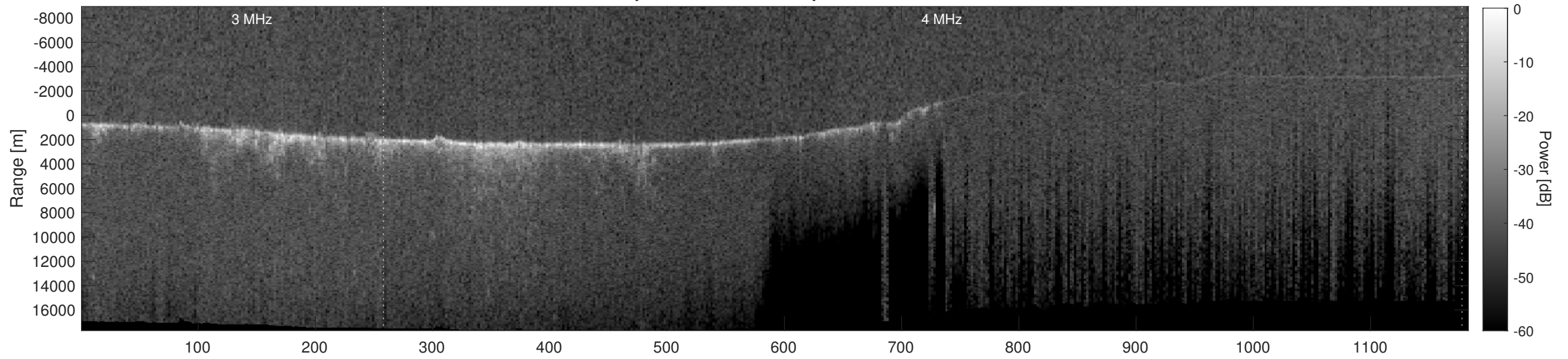
Orbit 9381, Depth-Corrected Cluttergram
