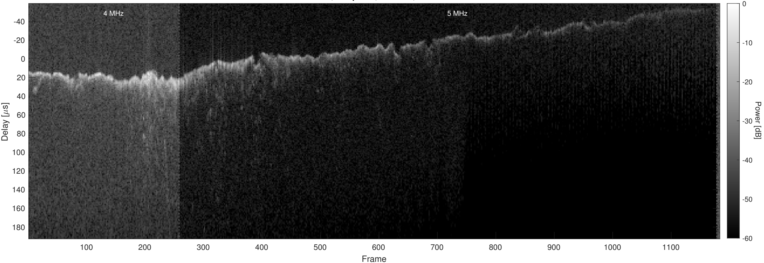
Orbit 9382, Chapman, Window, Channel 2
