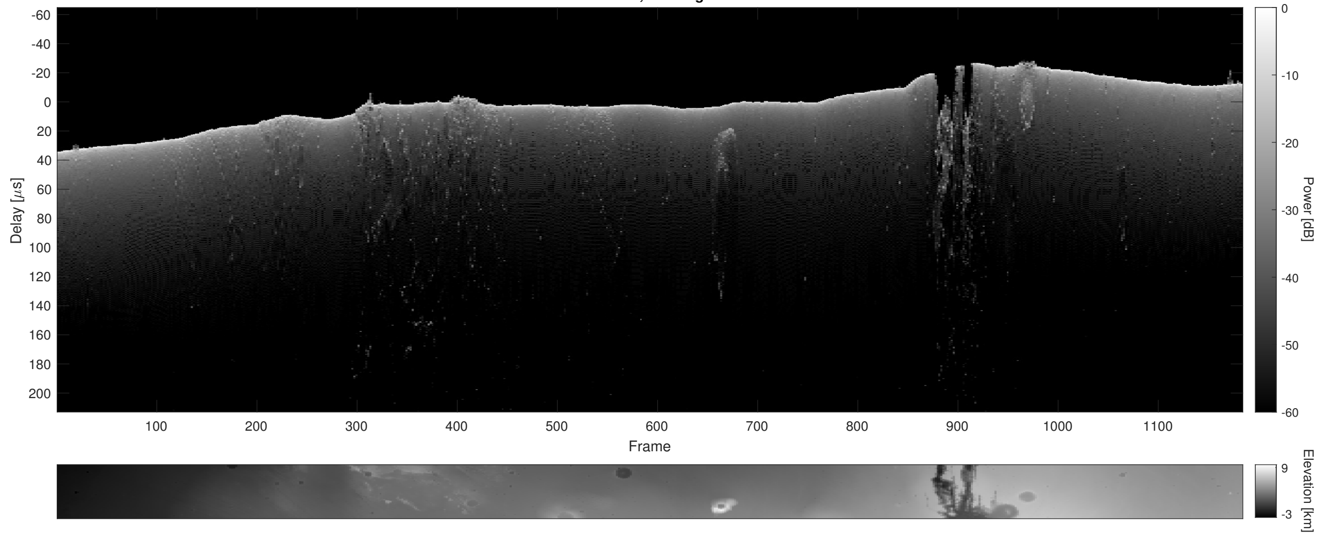
Orbit 9383, Cluttergram
