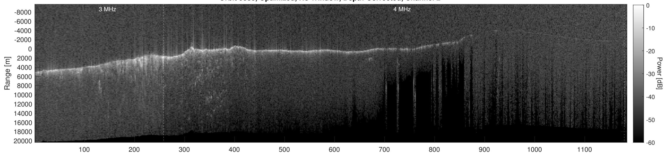
Orbit 9383, Depth-Corrected Cluttergram
