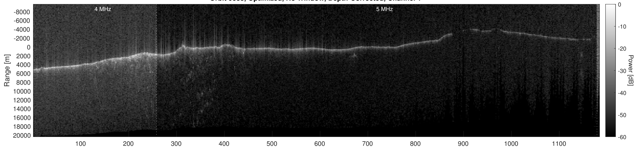
Orbit 9383, Optimized, No Window, Depth-Corrected, Channel 2
