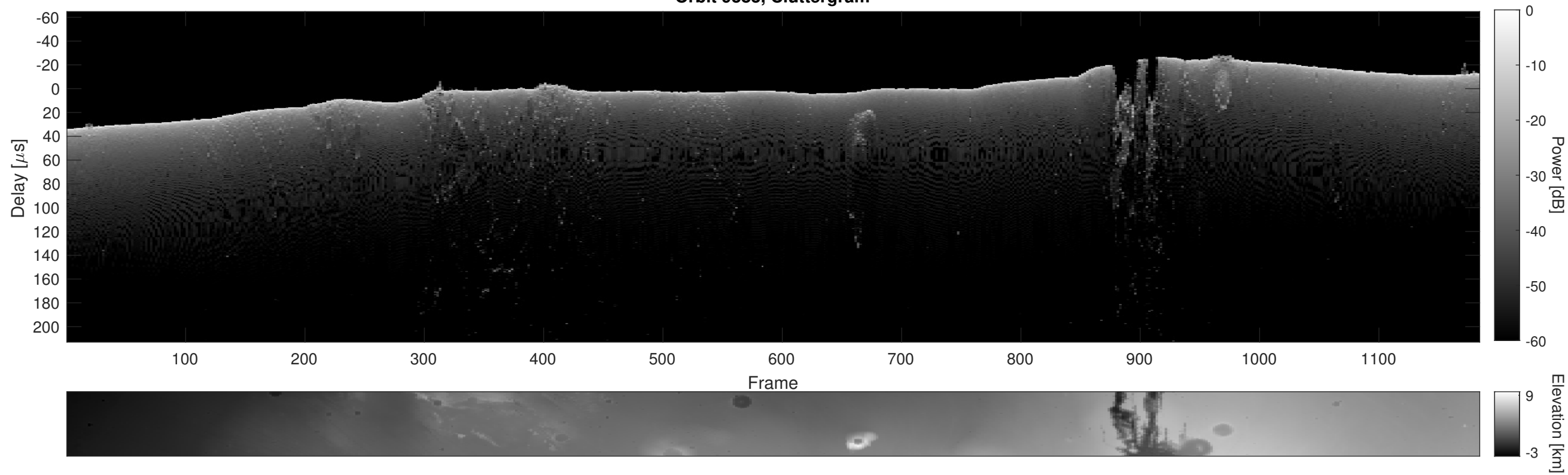
Orbit 9383, Cluttergram
