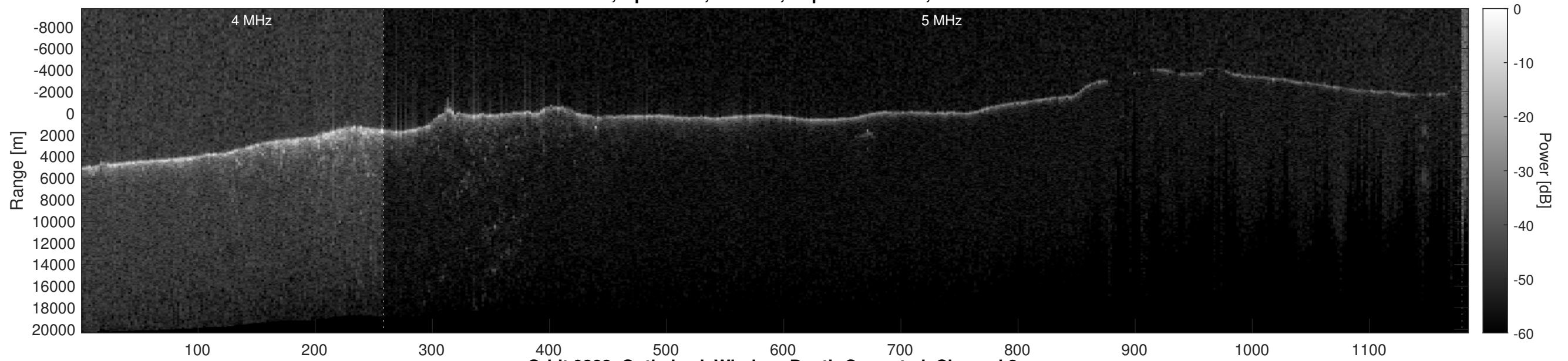
Orbit 9383, Optimized, Window, Depth-Corrected, Channel 2
