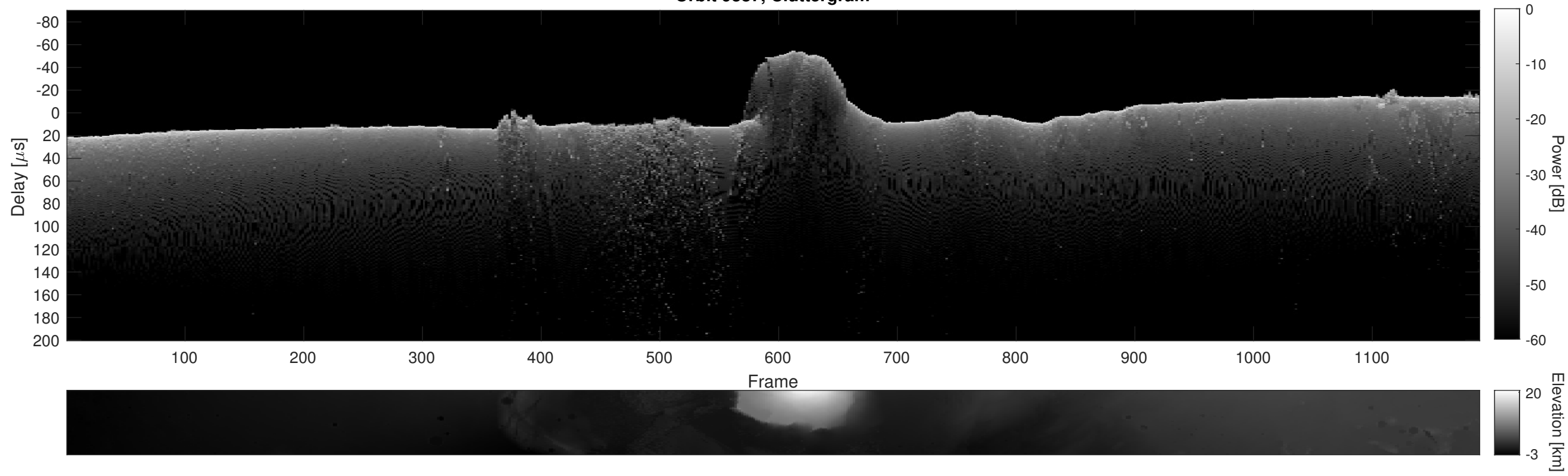
Orbit 9387, Cluttergram
