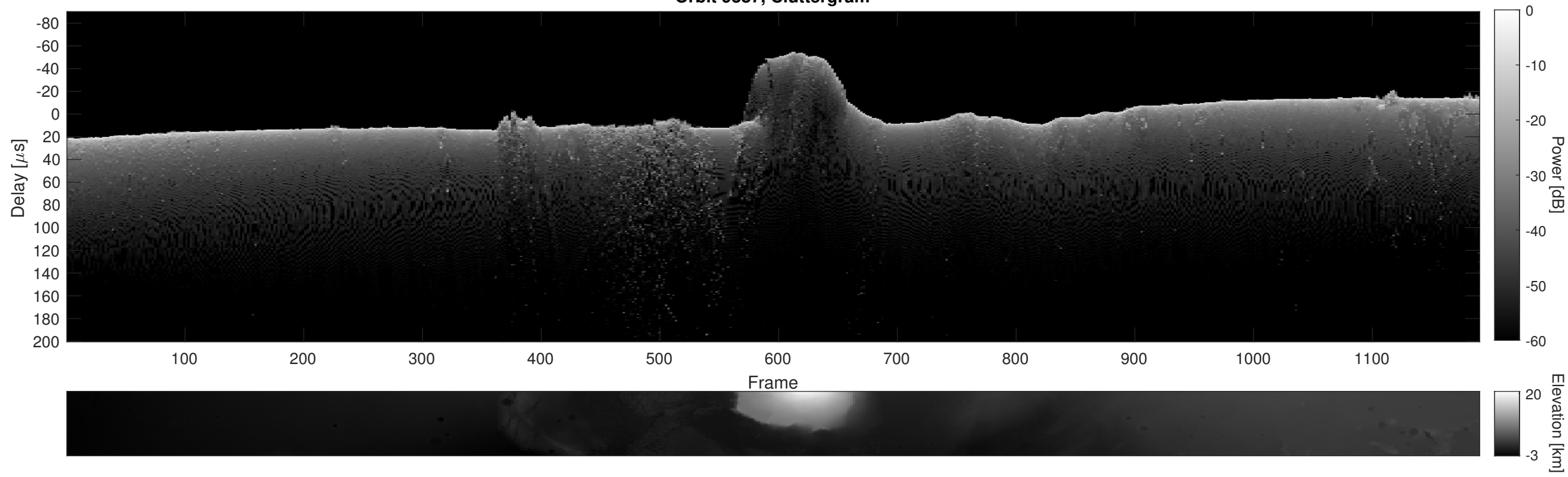
Orbit 9387, Cluttergram
