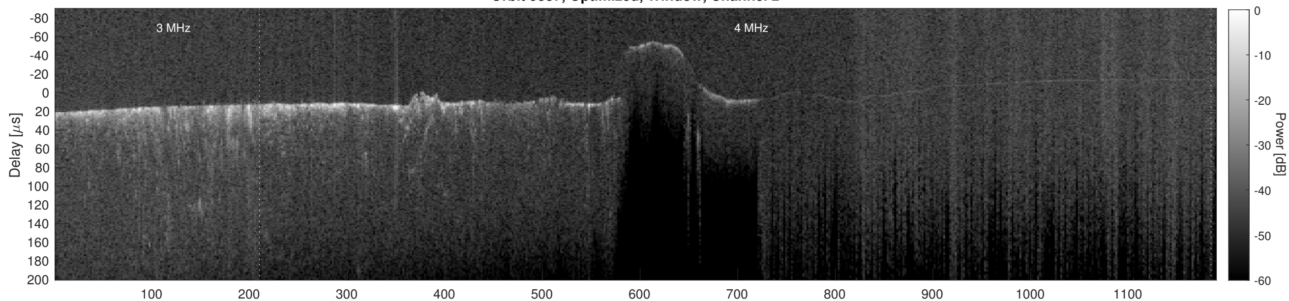
Orbit 9387, Cluttergram
