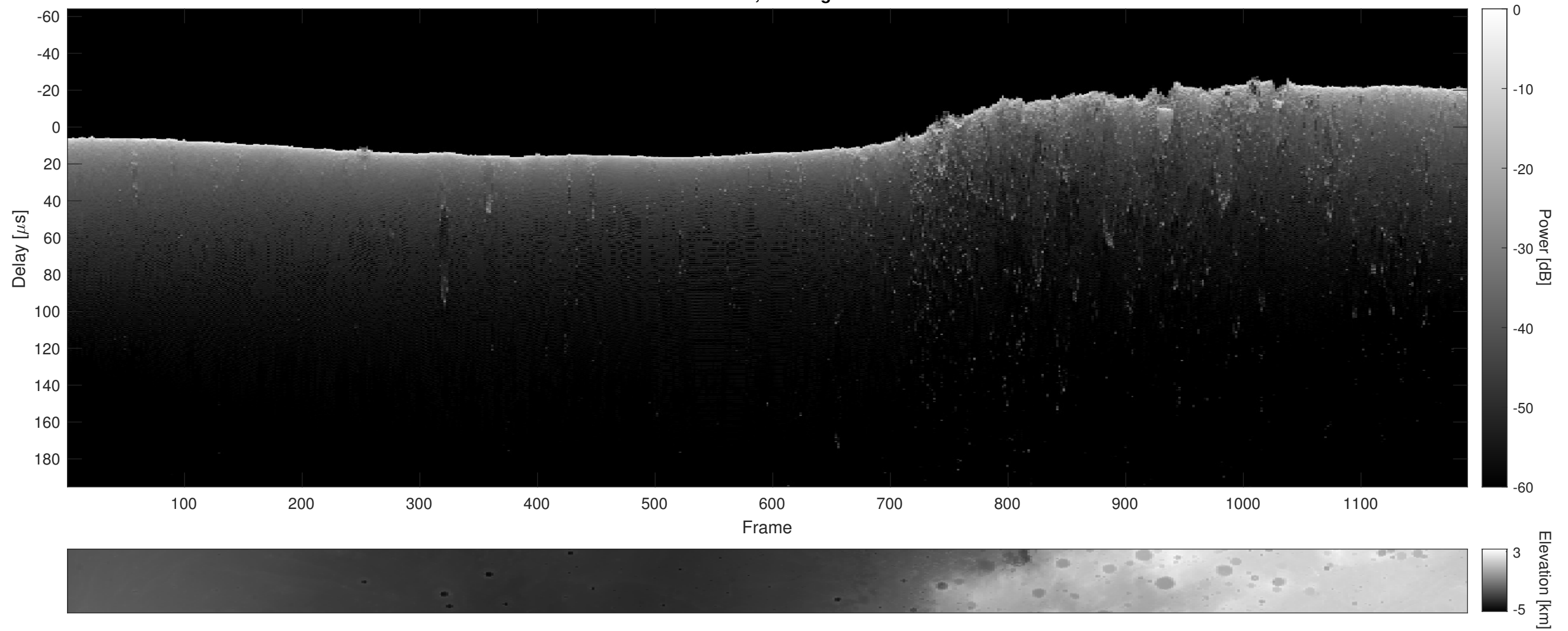
Orbit 9388, Cluttergram
