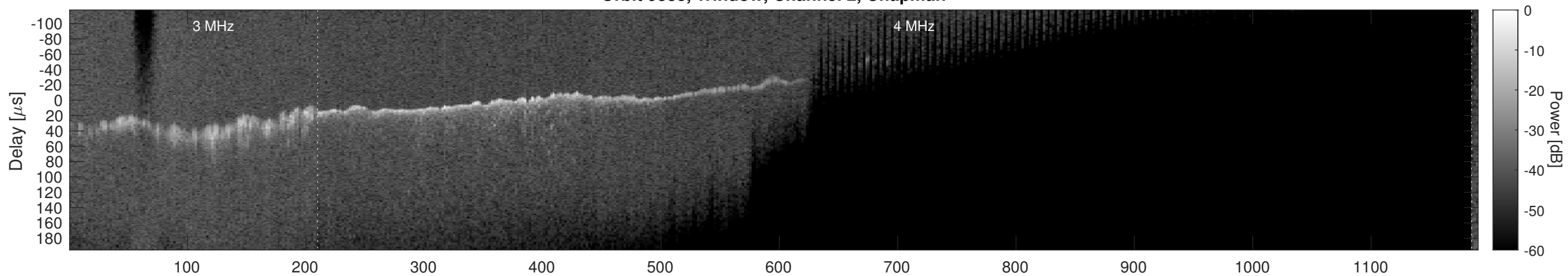
Orbit 9388, Window, Channel 2, Optimized
