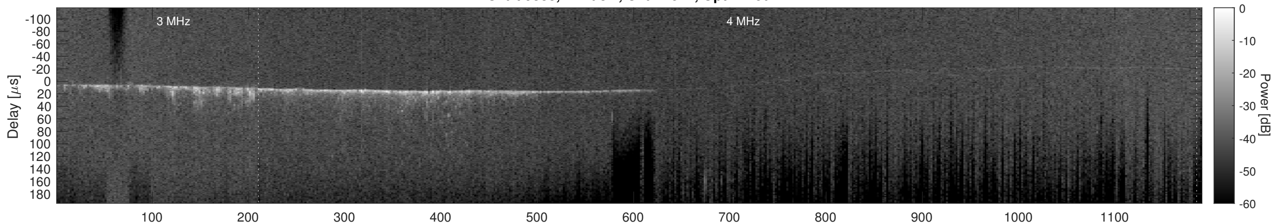
Orbit 9388, Cluttergram
