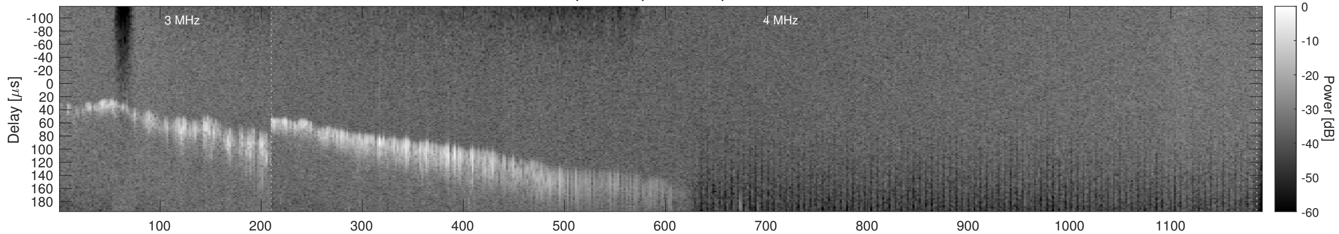
Orbit 9388, Window, Channel 2, Chapman
