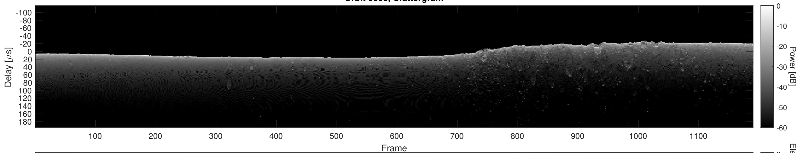
Orbit 9388, Cluttergram
