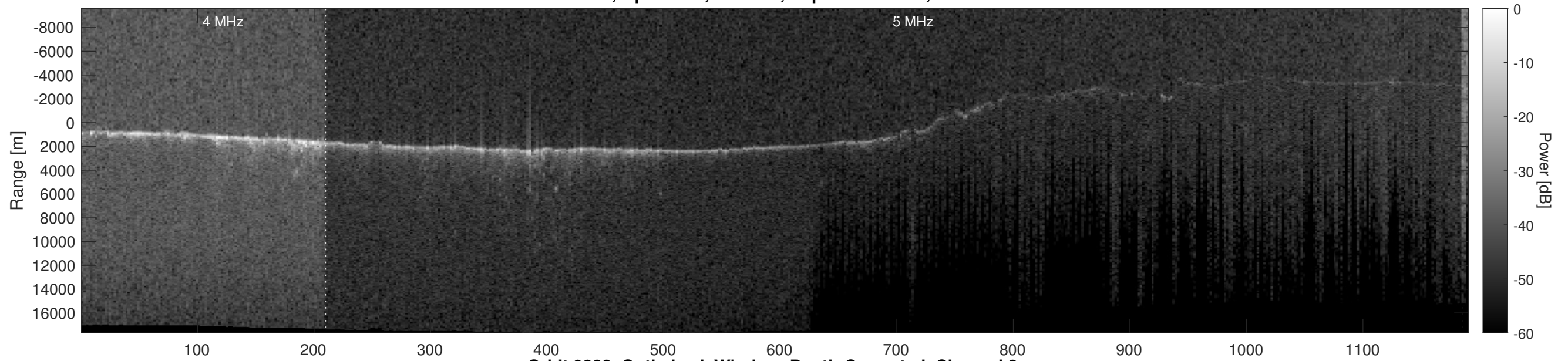
Orbit 9388, Optimized, Window, Depth-Corrected, Channel 2
