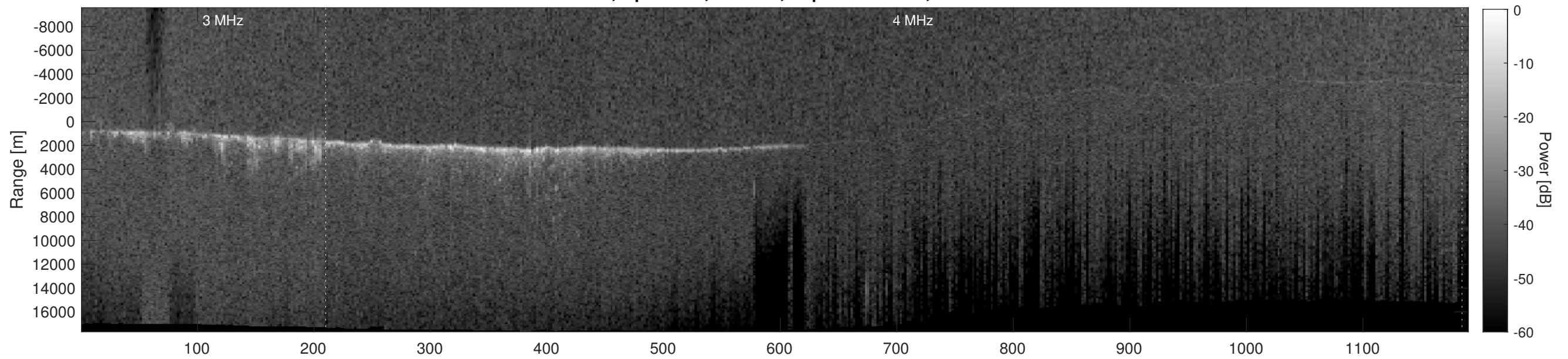
Orbit 9388, Depth-Corrected Cluttergram
