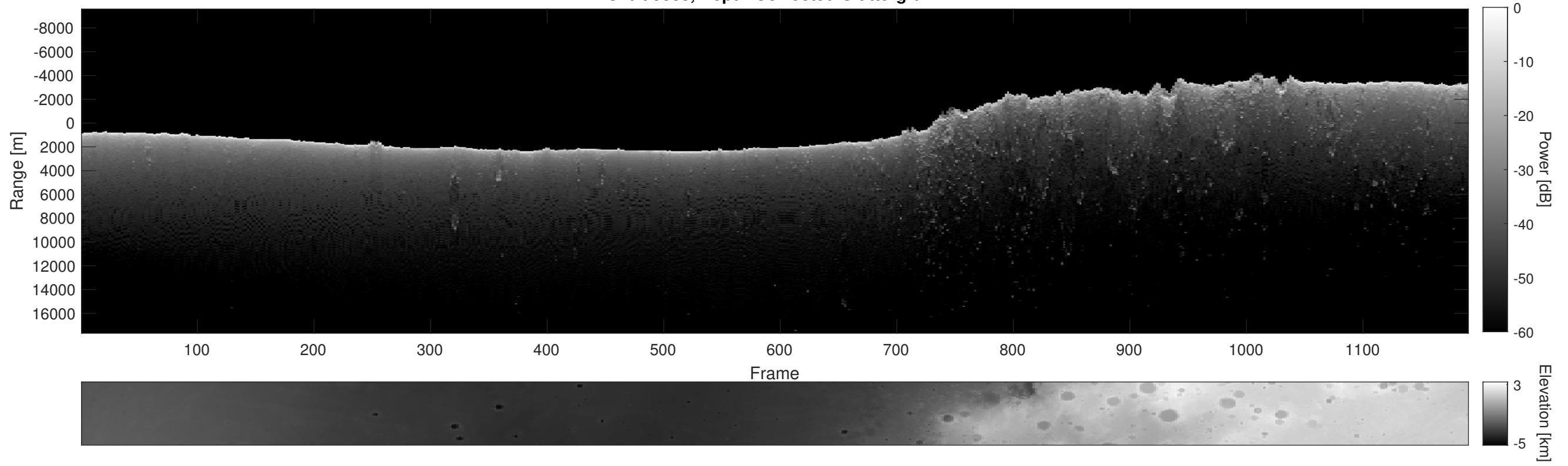
Orbit 9388, Depth-Corrected Cluttergram
