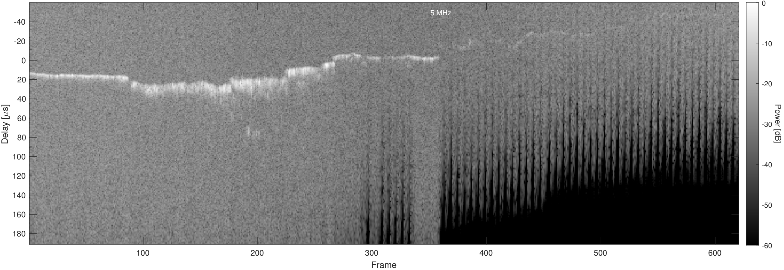
Orbit 9389, Chapman, Window, Channel 2
