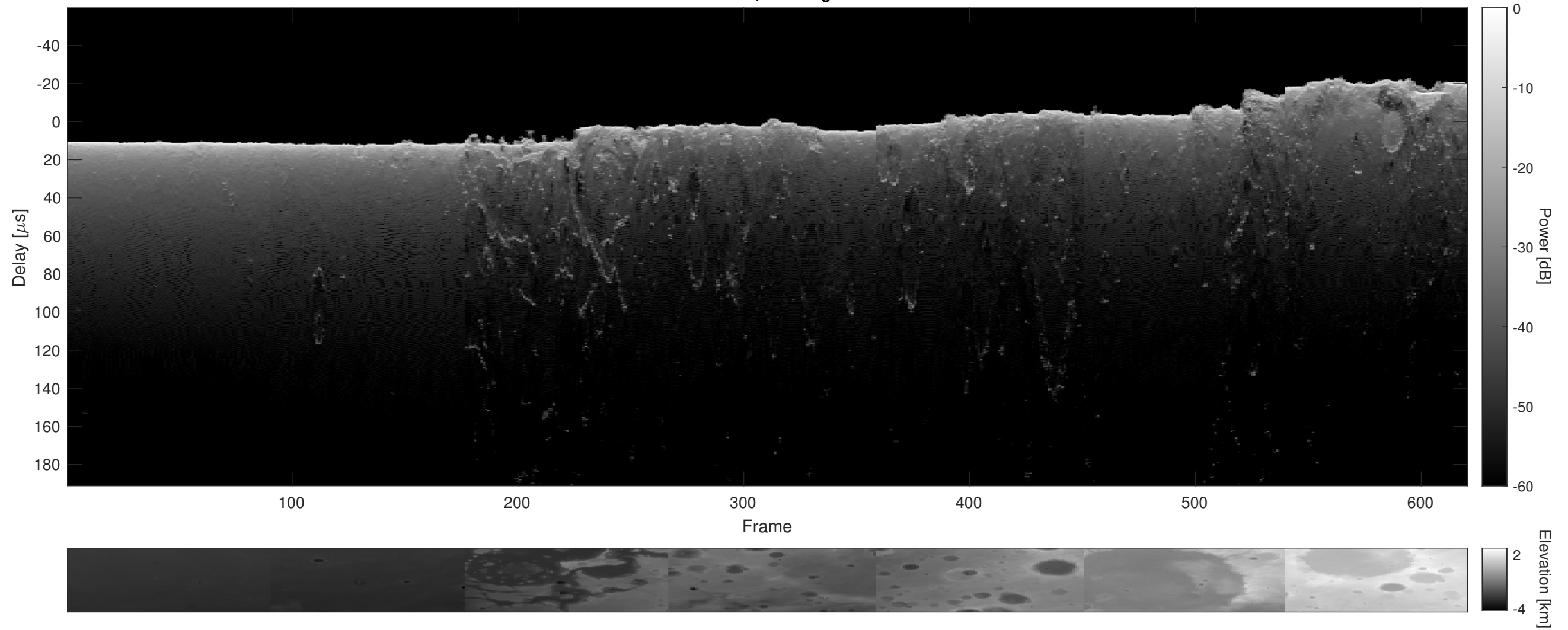
Orbit 9389, Cluttergram
