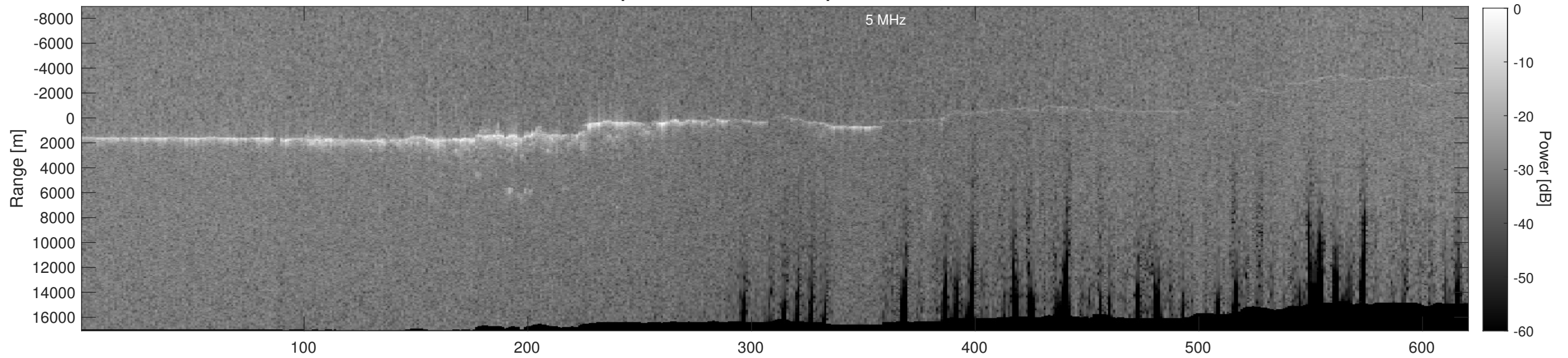
Orbit 9389, Depth-Corrected Cluttergram
