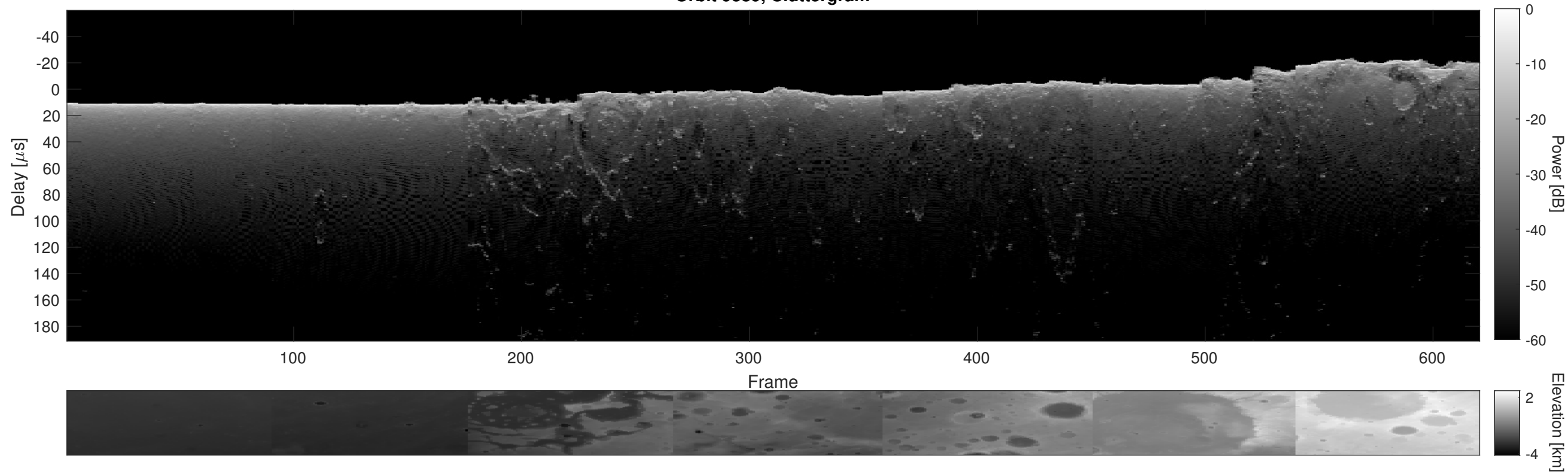
Orbit 9389, Cluttergram
