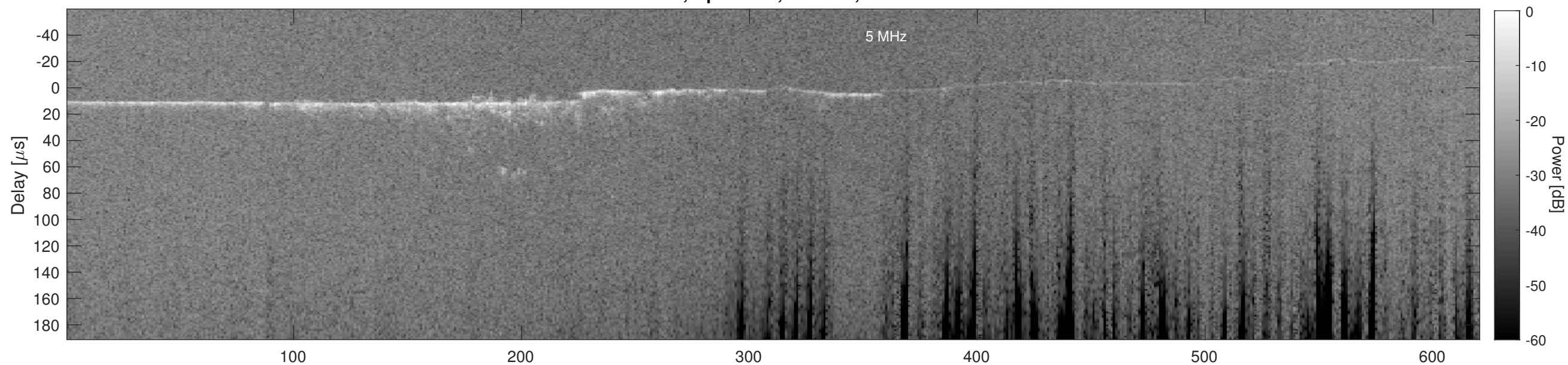
Orbit 9389, Cluttergram
