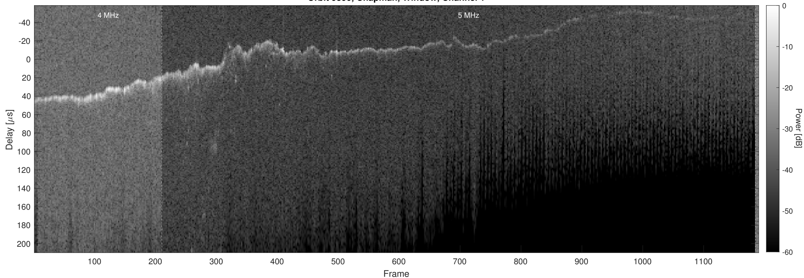
Orbit 9390, Chapman, Window, Channel 2
