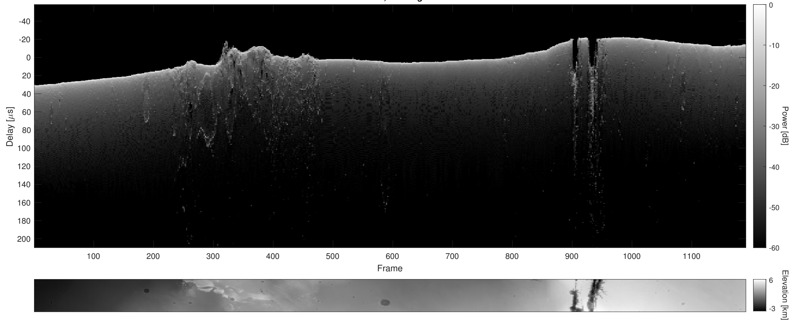
Orbit 9390, Cluttergram
