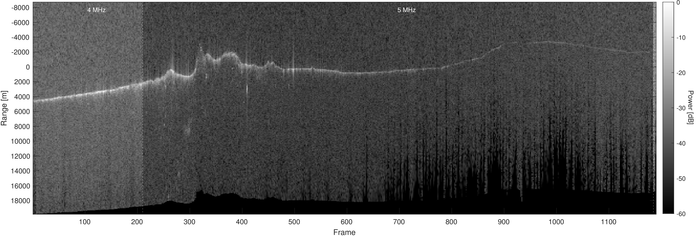
Orbit 9390, Optimized, No Window, Depth-Corrected, Channel 2
