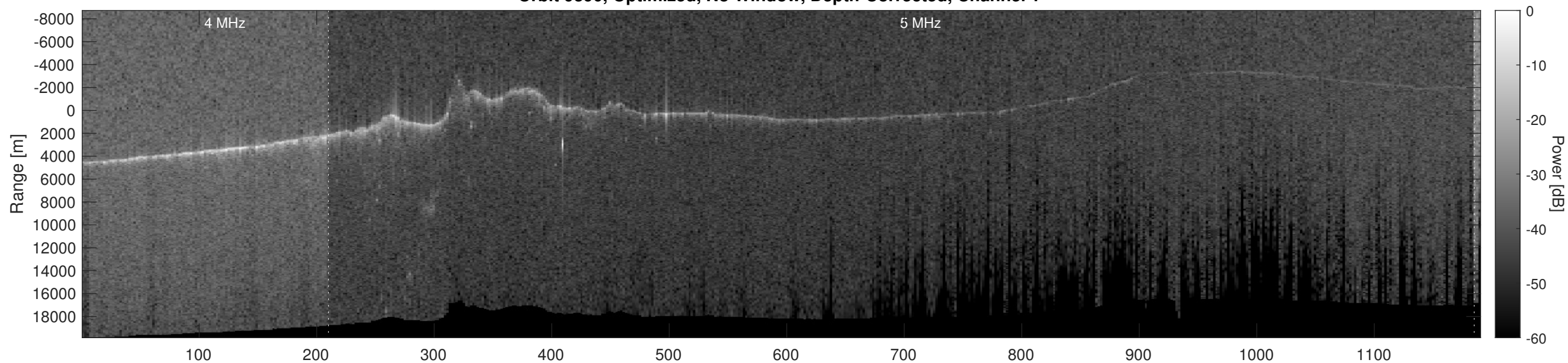
Orbit 9390, Optimized, No Window, Depth-Corrected, Channel 2
