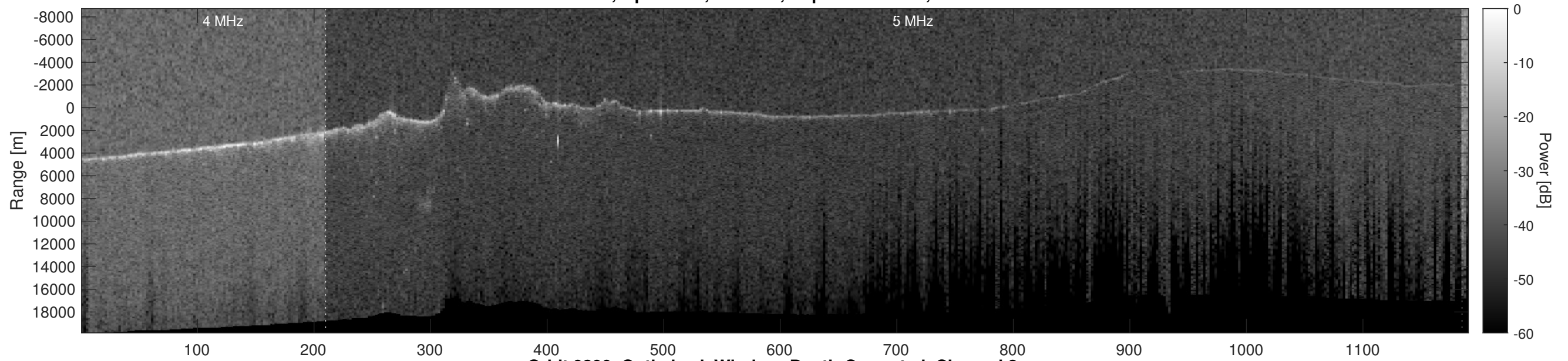
Orbit 9390, Optimized, Window, Depth-Corrected, Channel 2
