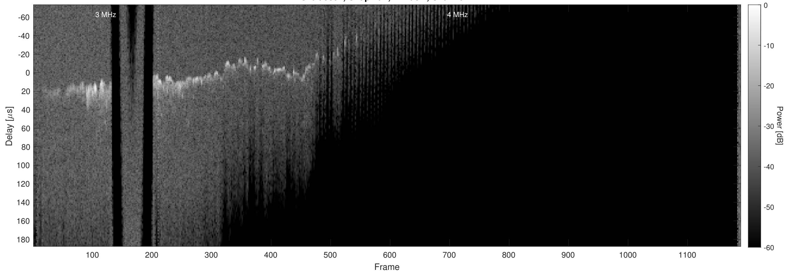
Orbit 9391, Chapman, Window, Channel 2
