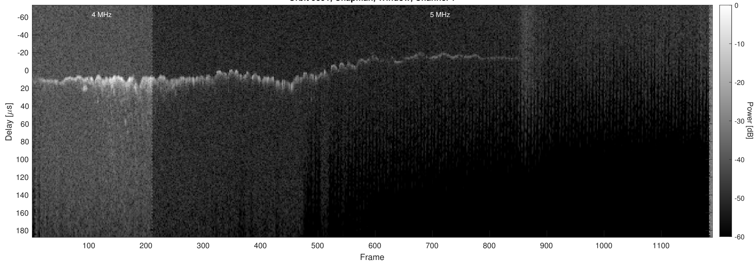
Orbit 9391, Chapman, Window, Channel 2
