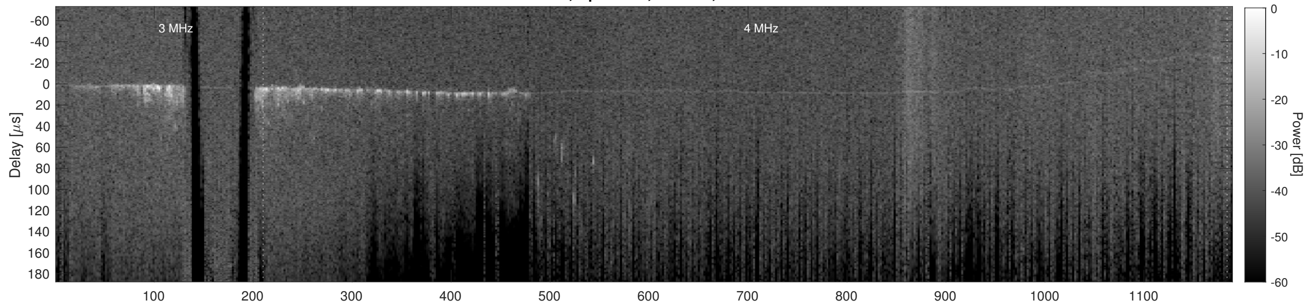
Orbit 9391, Cluttergram
