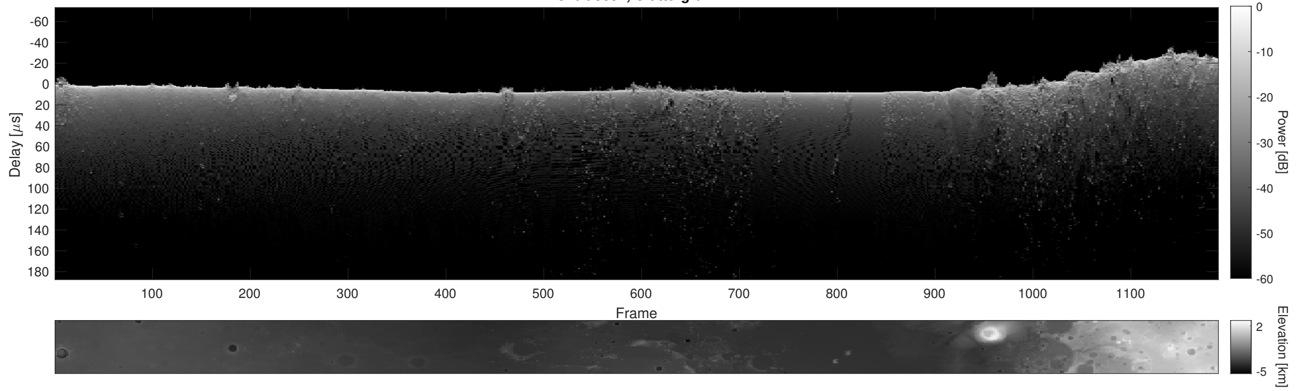
Orbit 9391, Cluttergram
