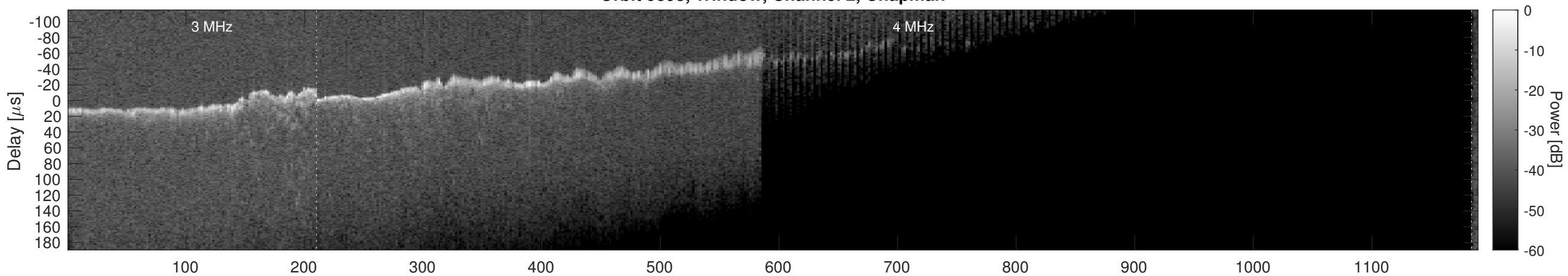
Orbit 9393, Window, Channel 2, Optimized
