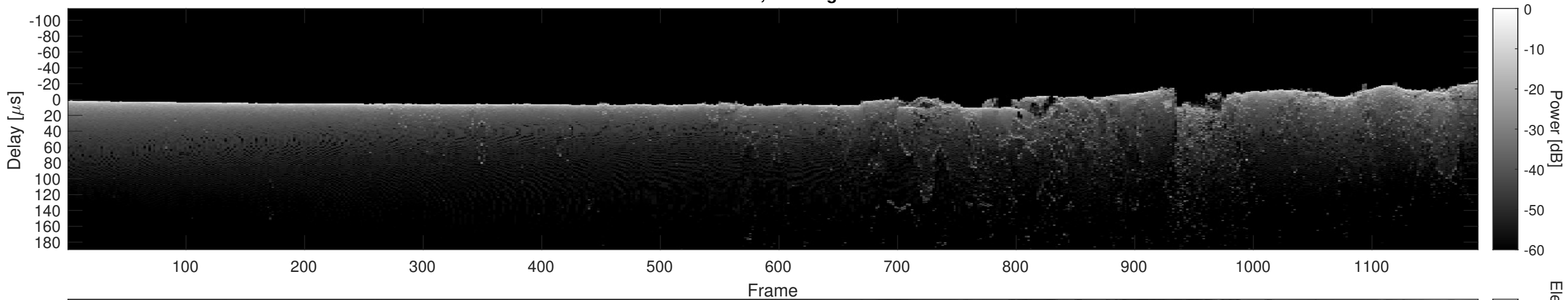
Orbit 9393, Cluttergram
