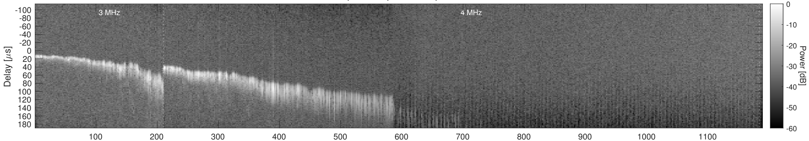
Orbit 9393, Window, Channel 2, Chapman
