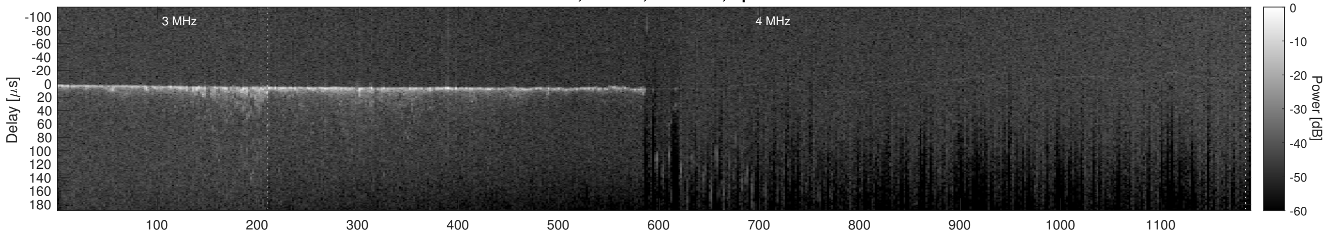
Orbit 9393, Cluttergram
