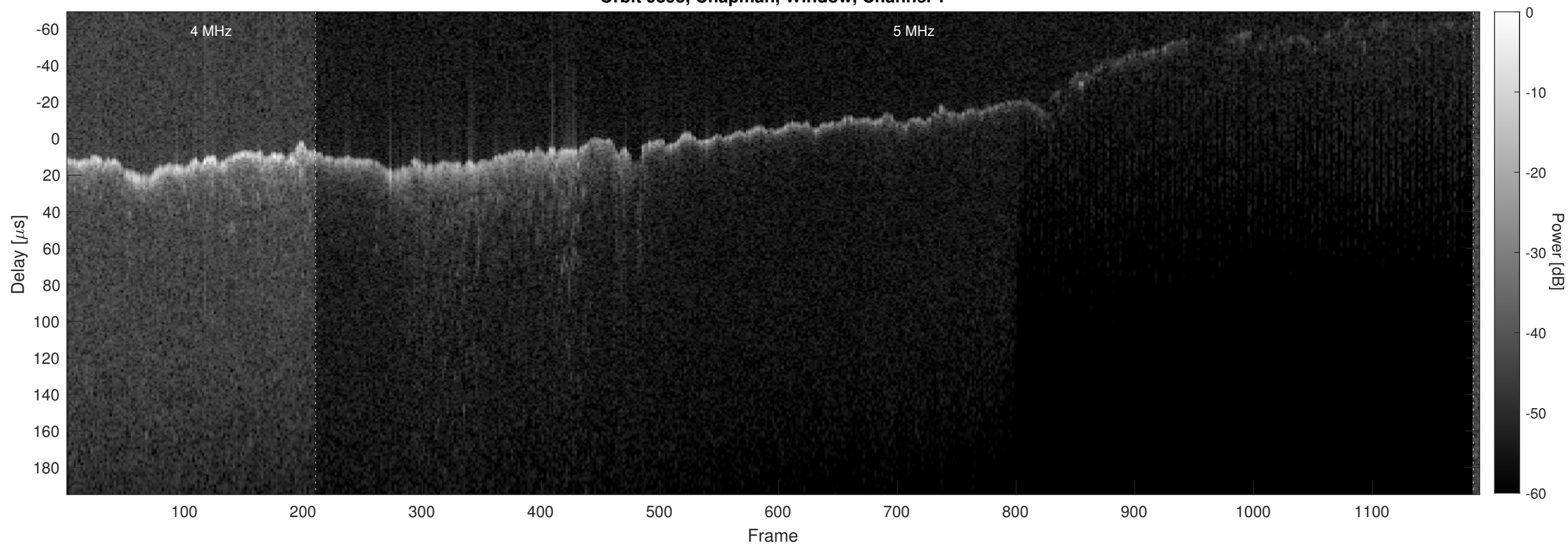
Orbit 9395, Chapman, Window, Channel 2
