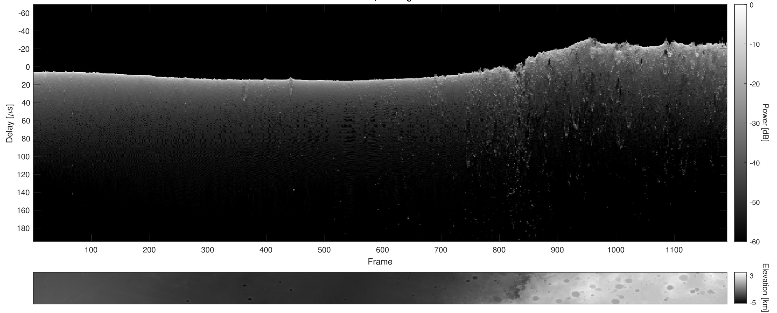
Orbit 9395, Cluttergram
