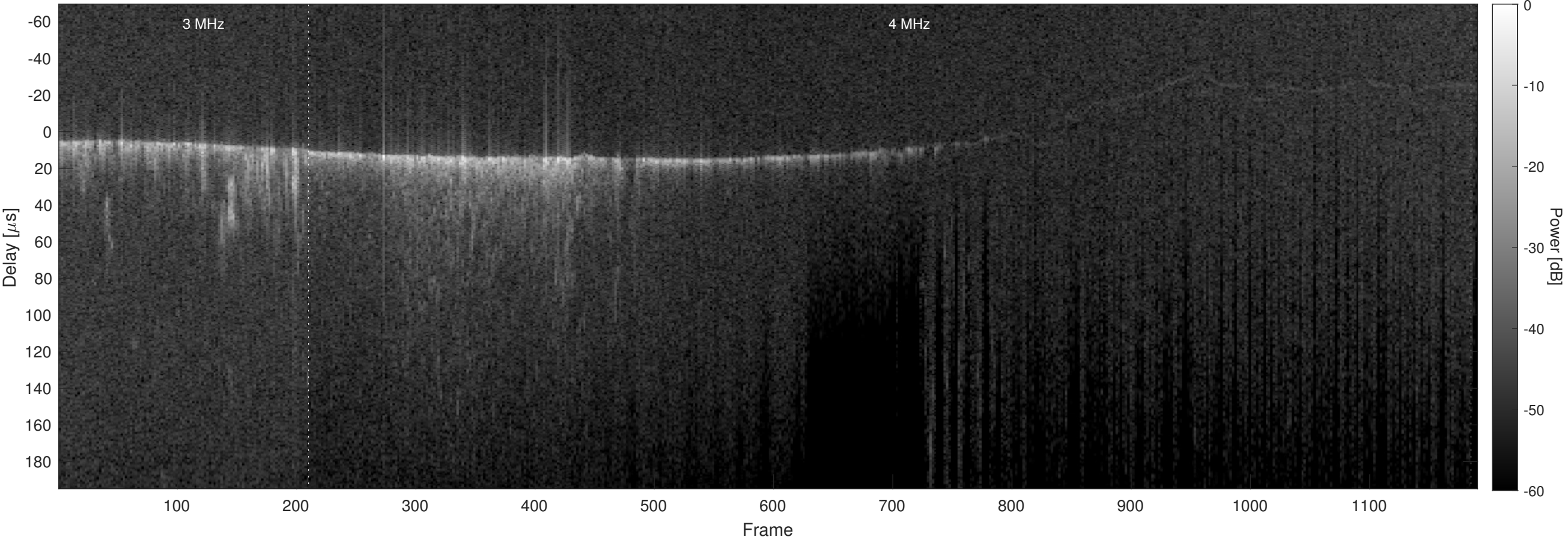
Orbit 9395, Optimized, No Window, Channel 2
