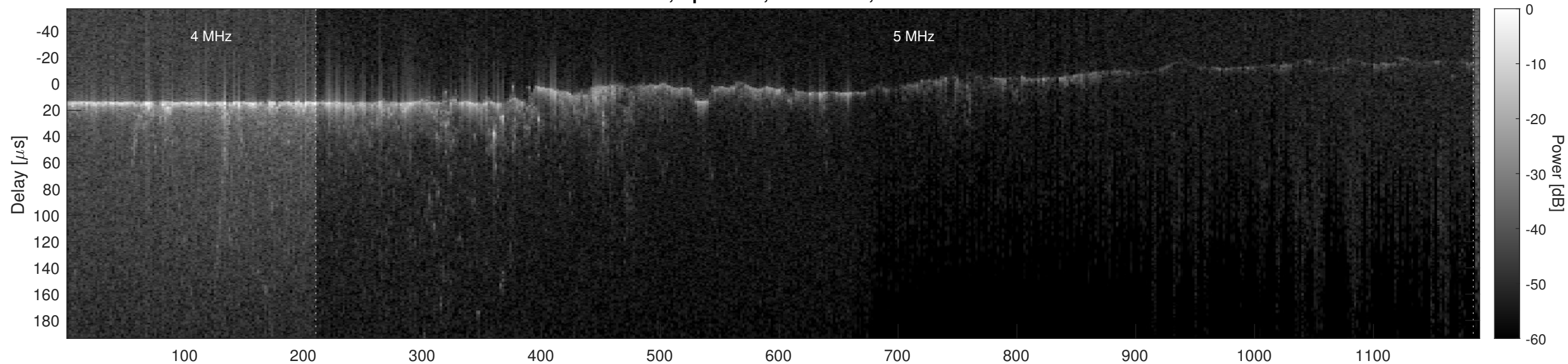
Orbit 9396, Optimized, No Window, Channel 2
