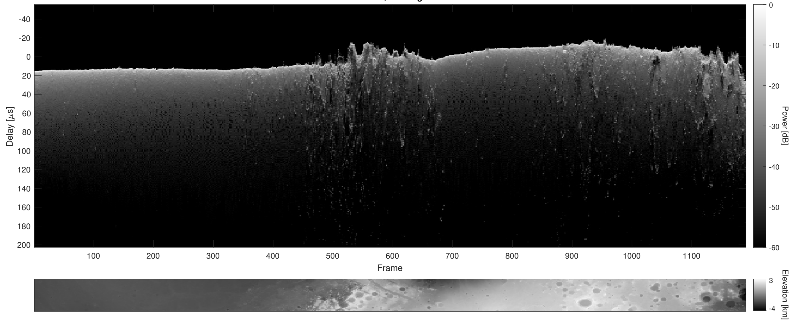
Orbit 9399, Cluttergram
