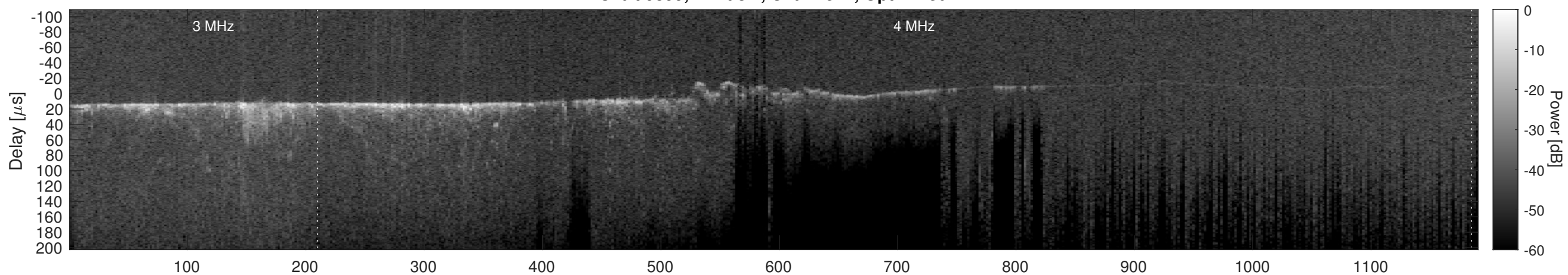
Orbit 9399, Cluttergram
