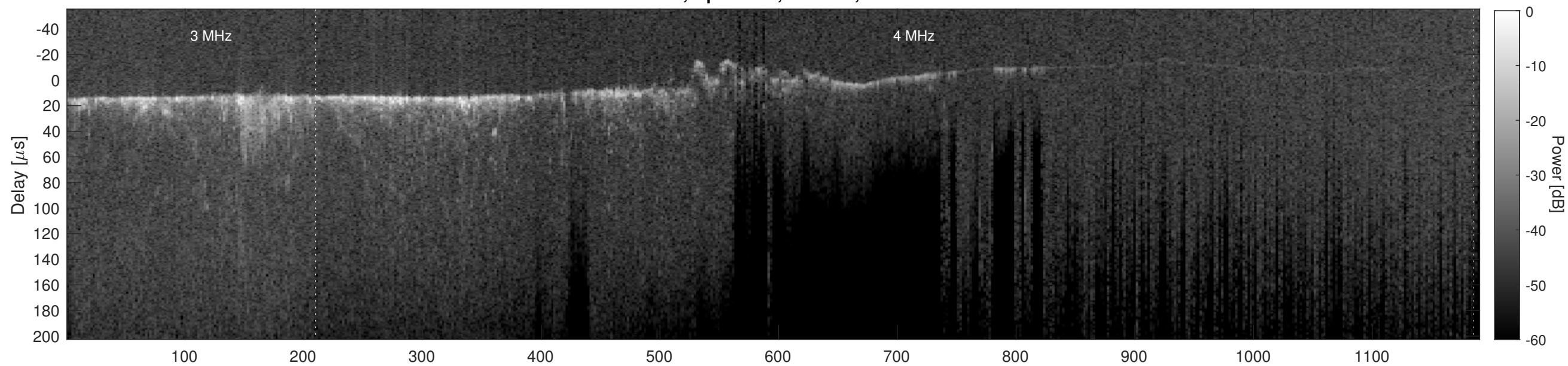
Orbit 9399, Cluttergram
