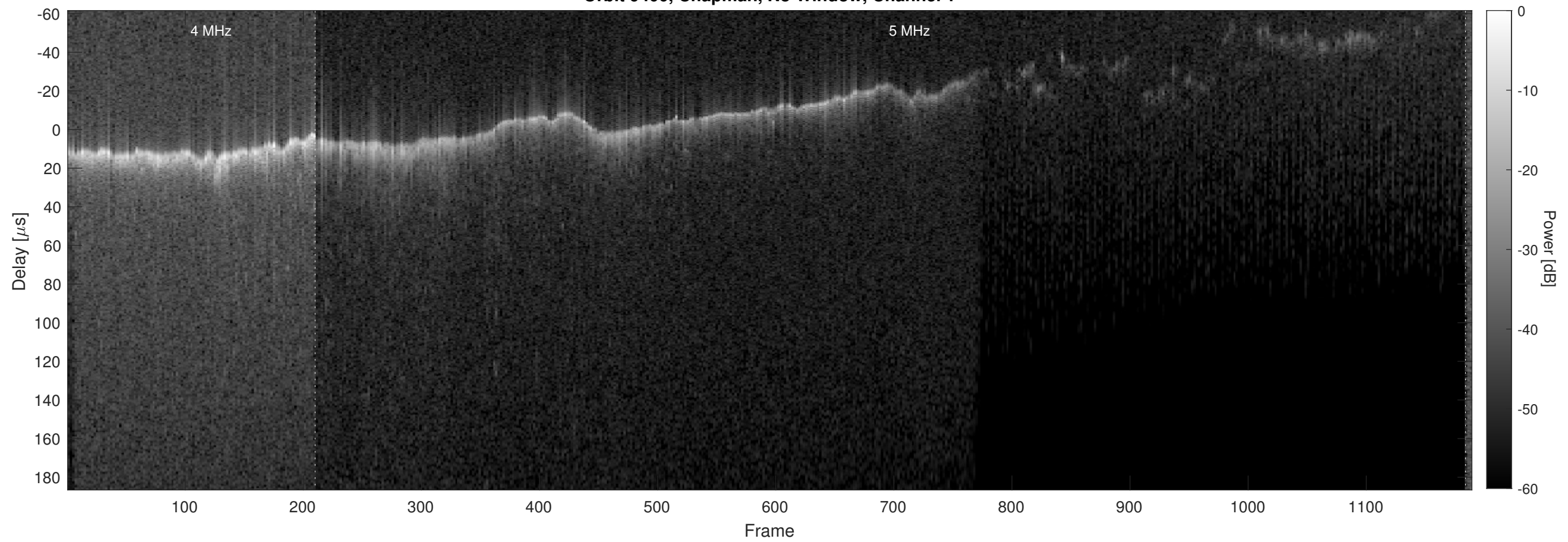
Orbit 9400, Chapman, No Window, Channel 2
