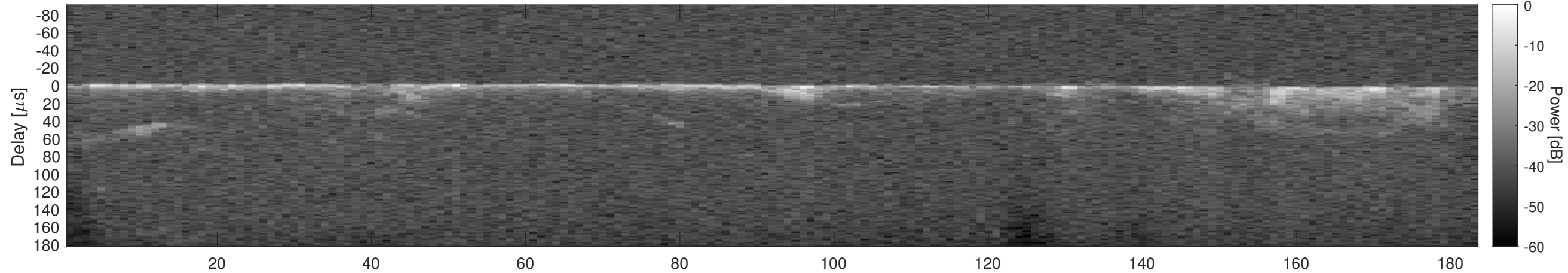
Orbit 9402, Cluttergram
