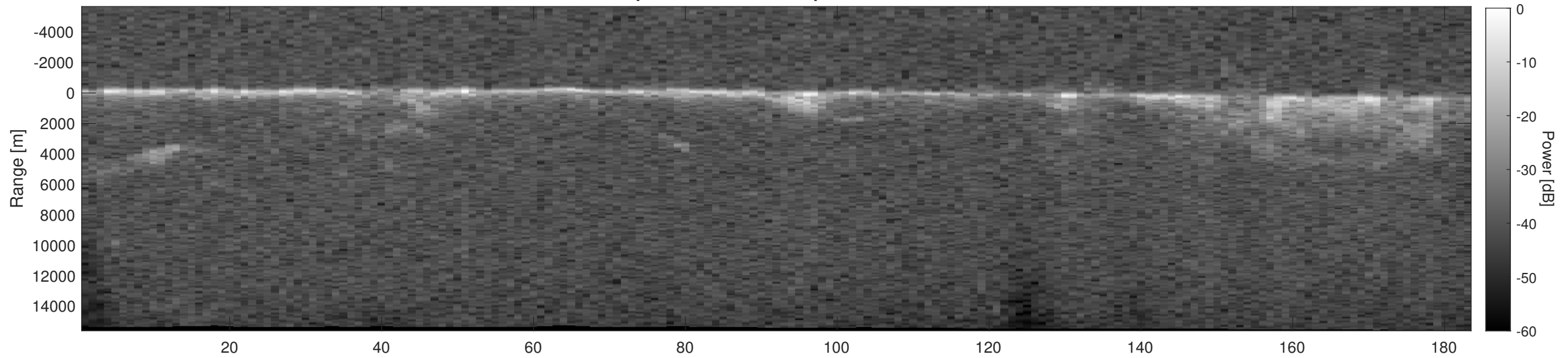
Orbit 9402, Depth-Corrected Cluttergram
