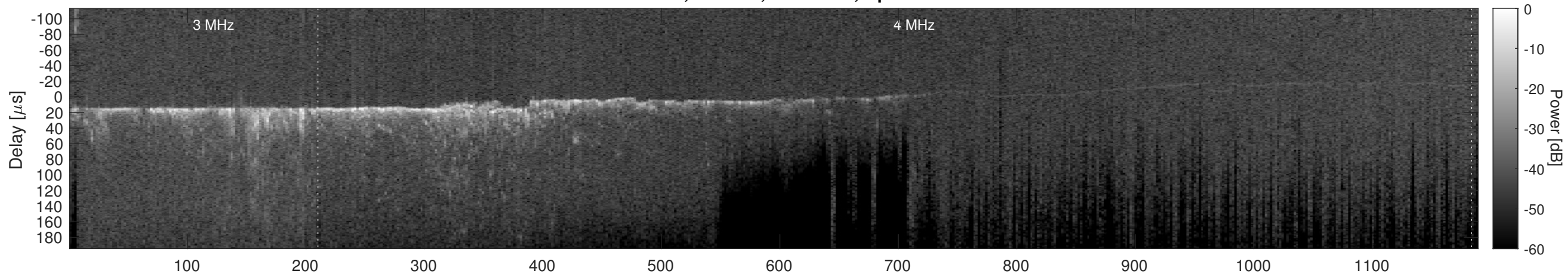
Orbit 9403, Cluttergram
