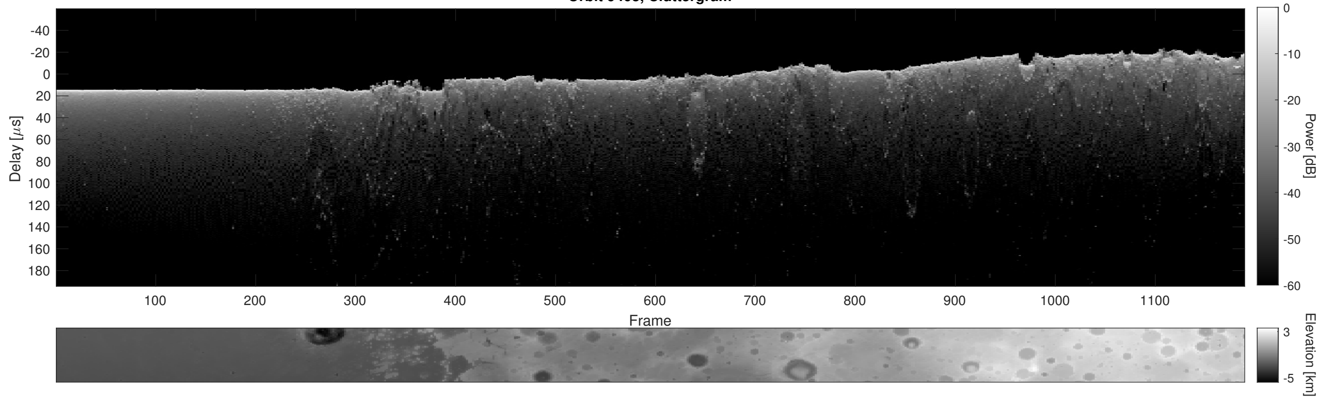
Orbit 9403, Cluttergram
