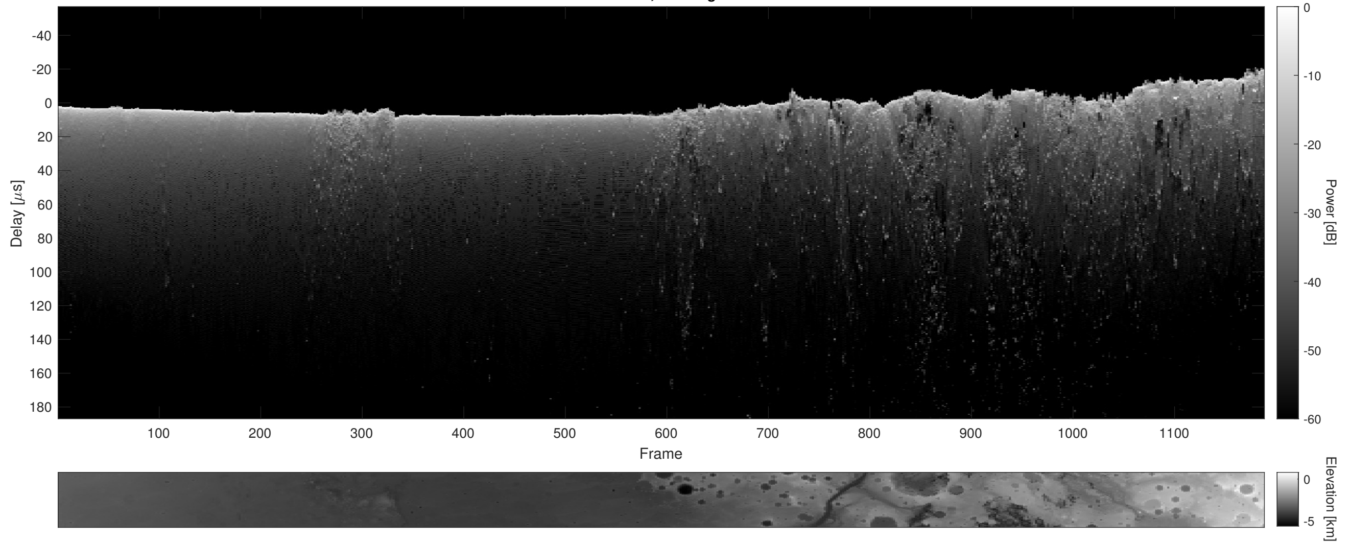
Orbit 9407, Cluttergram
