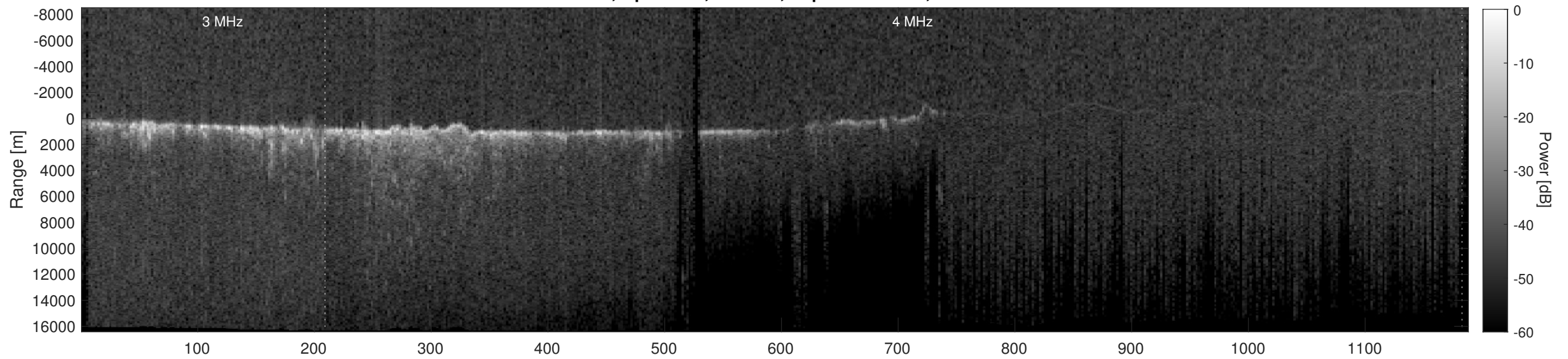
Orbit 9407, Depth-Corrected Cluttergram
