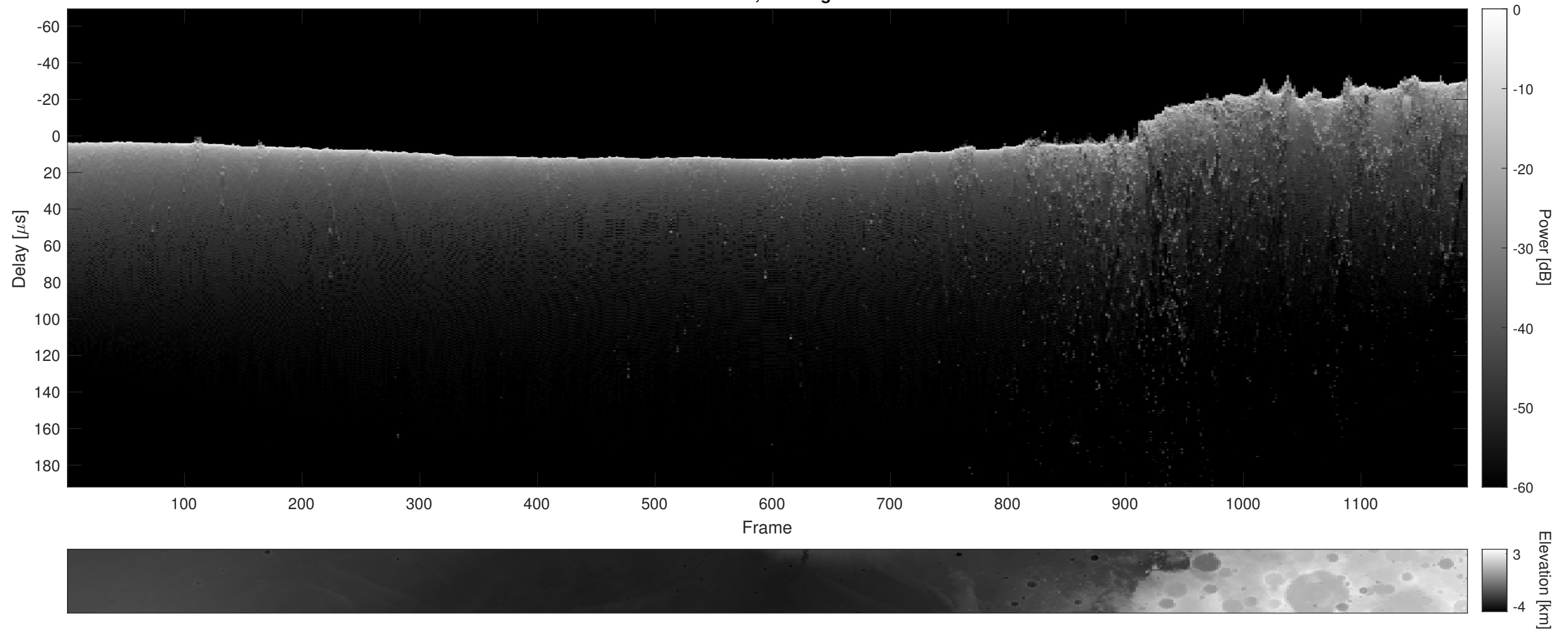
Orbit 9409, Cluttergram
