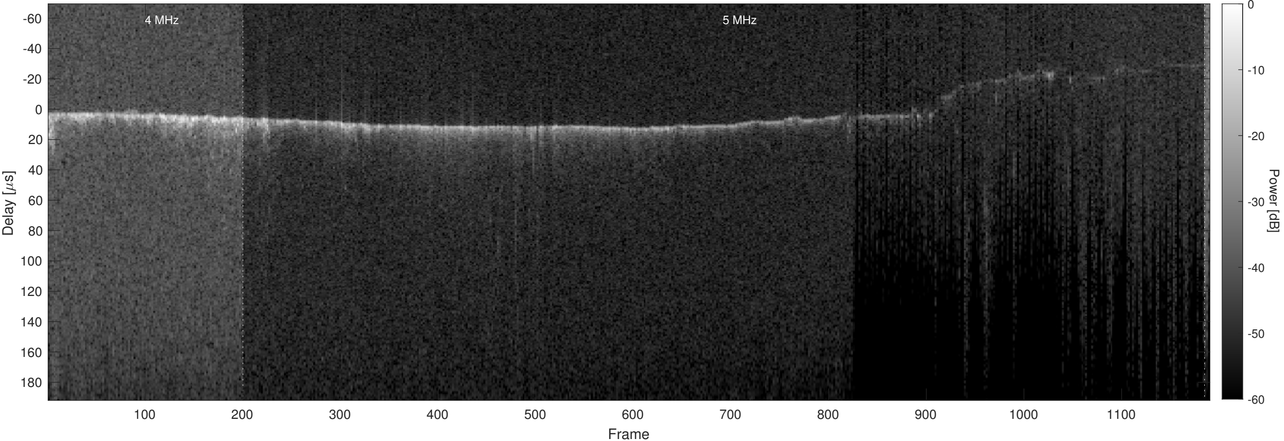
Orbit 9409, Optimized, Window, Channel 2
