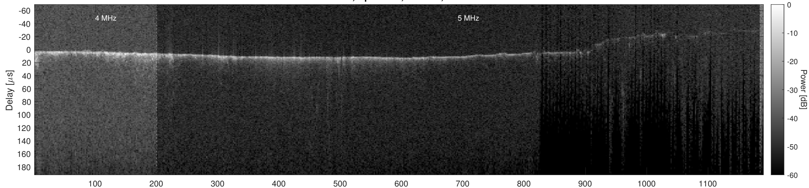
Orbit 9409, Optimized, Window, Channel 2
