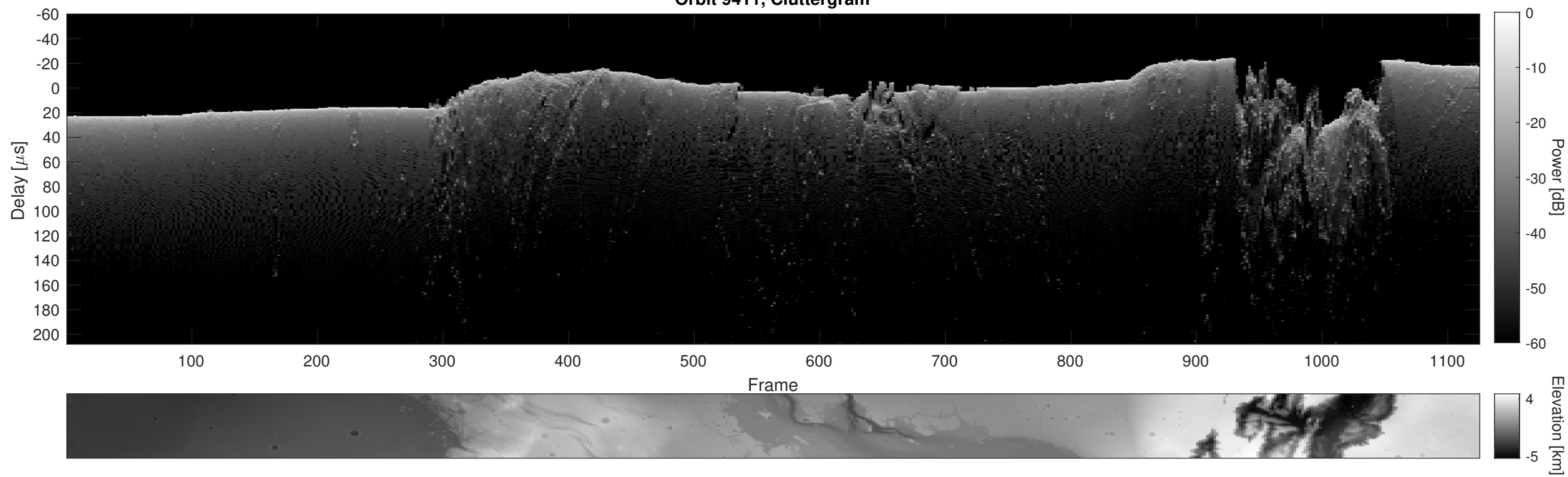
Orbit 9411, Cluttergram
