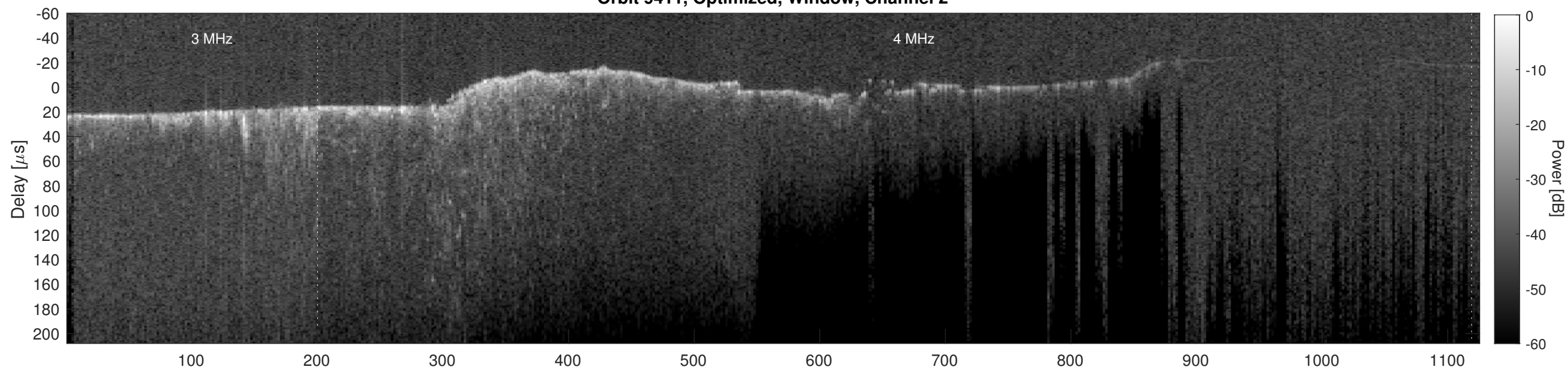
Orbit 9411, Cluttergram
