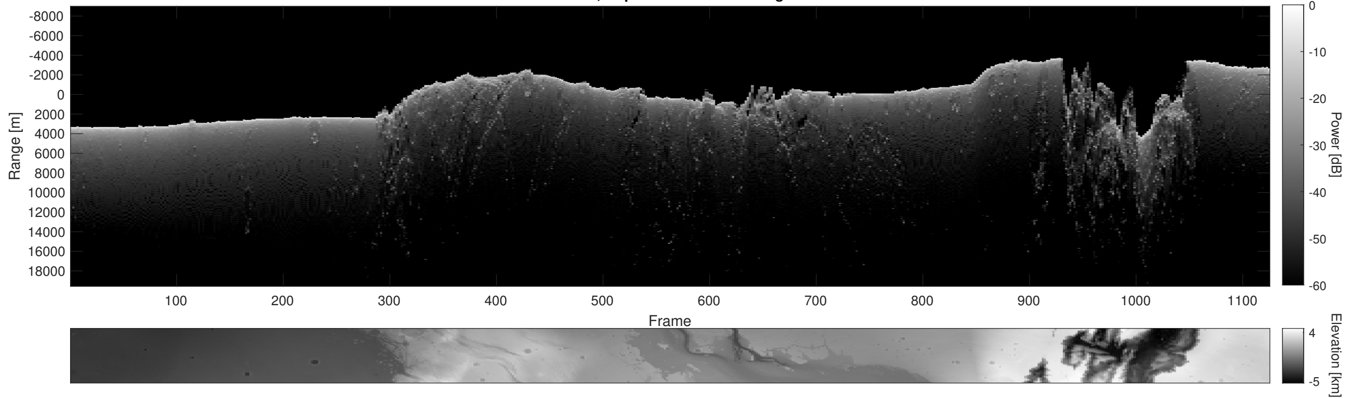
Orbit 9411, Depth-Corrected Cluttergram
