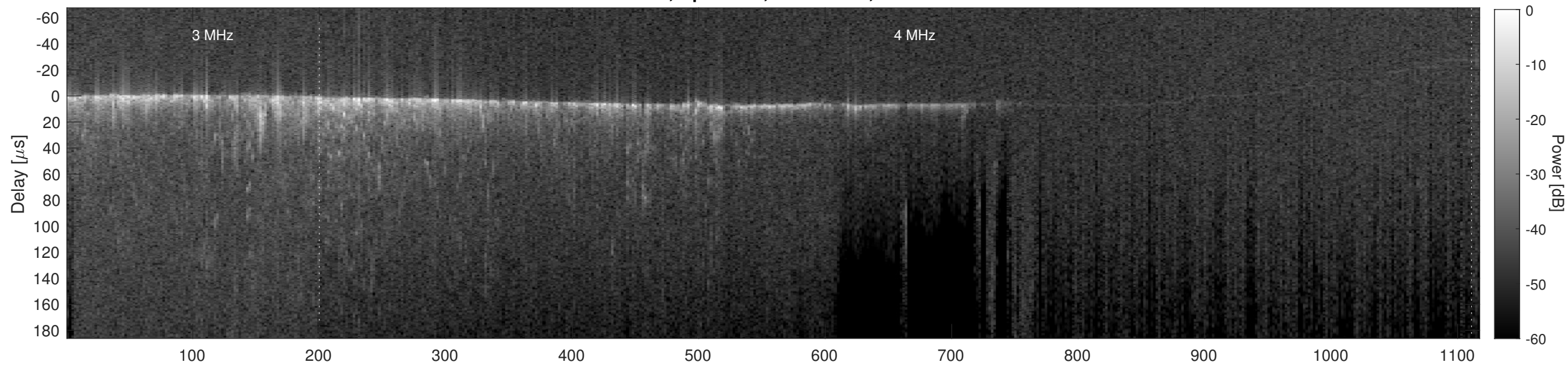
Orbit 9412, Cluttergram
