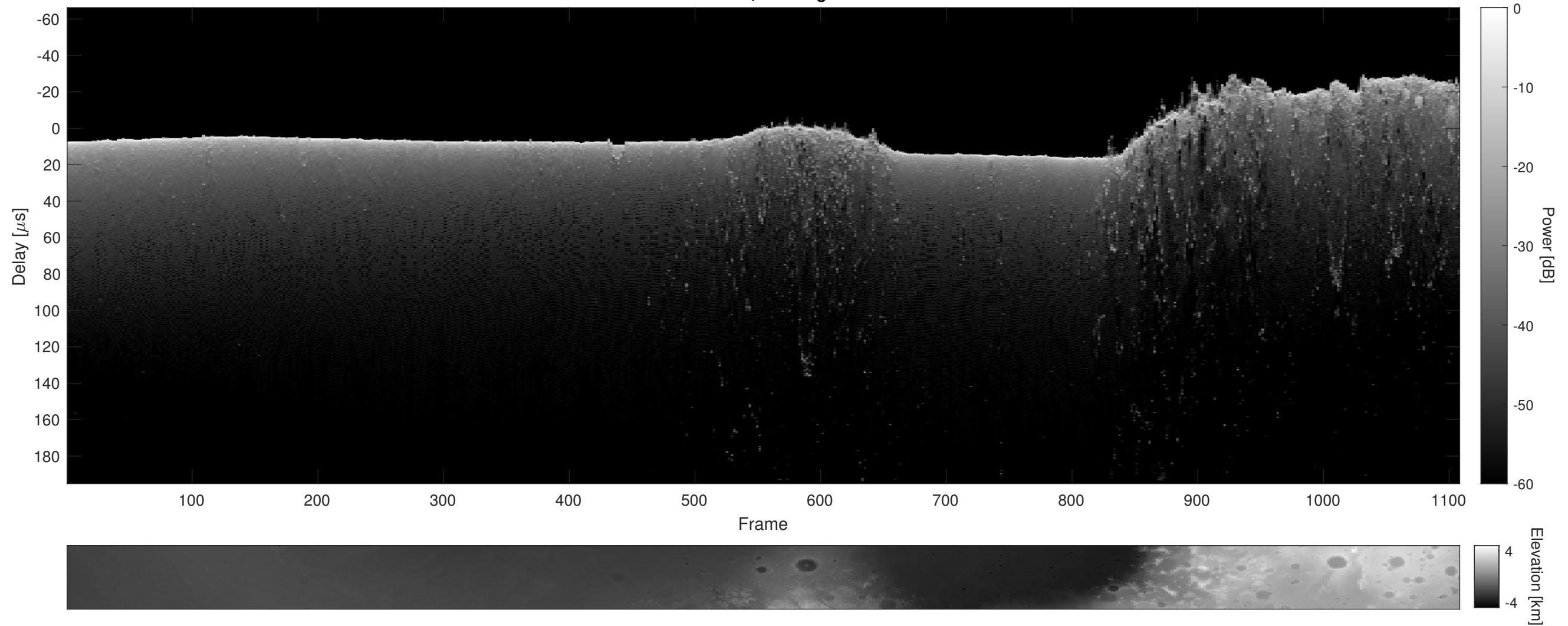
Orbit 9413, Cluttergram
