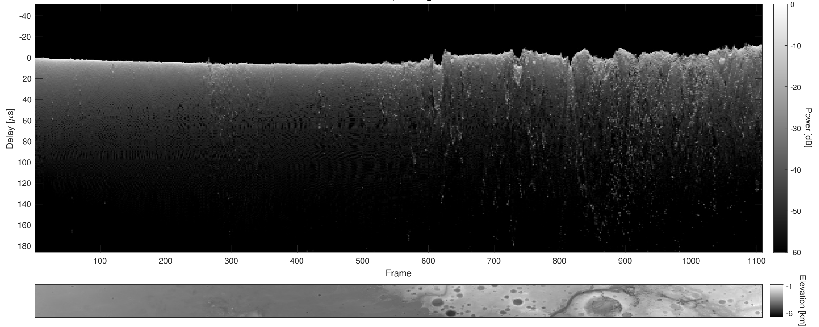
Orbit 9414, Cluttergram
