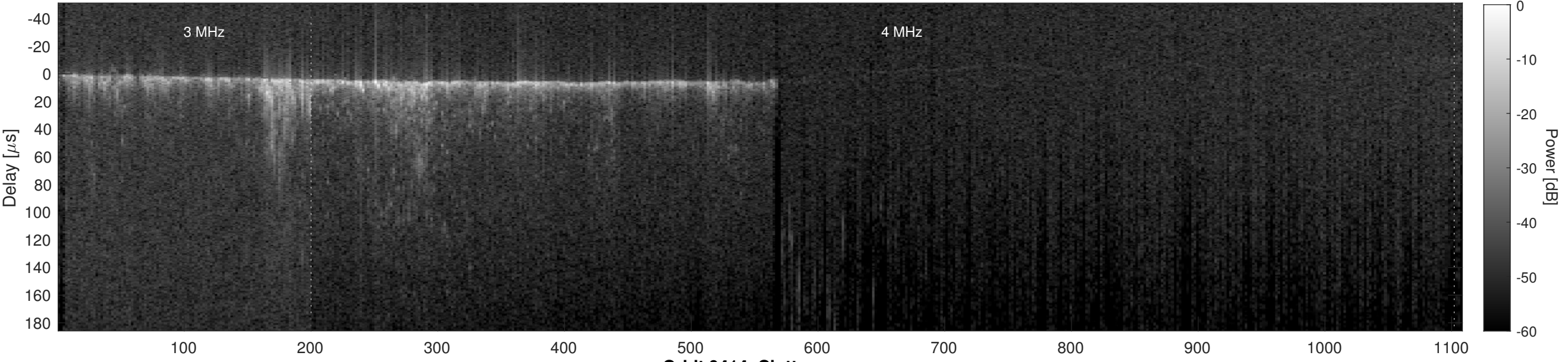
Orbit 9414, Cluttergram
