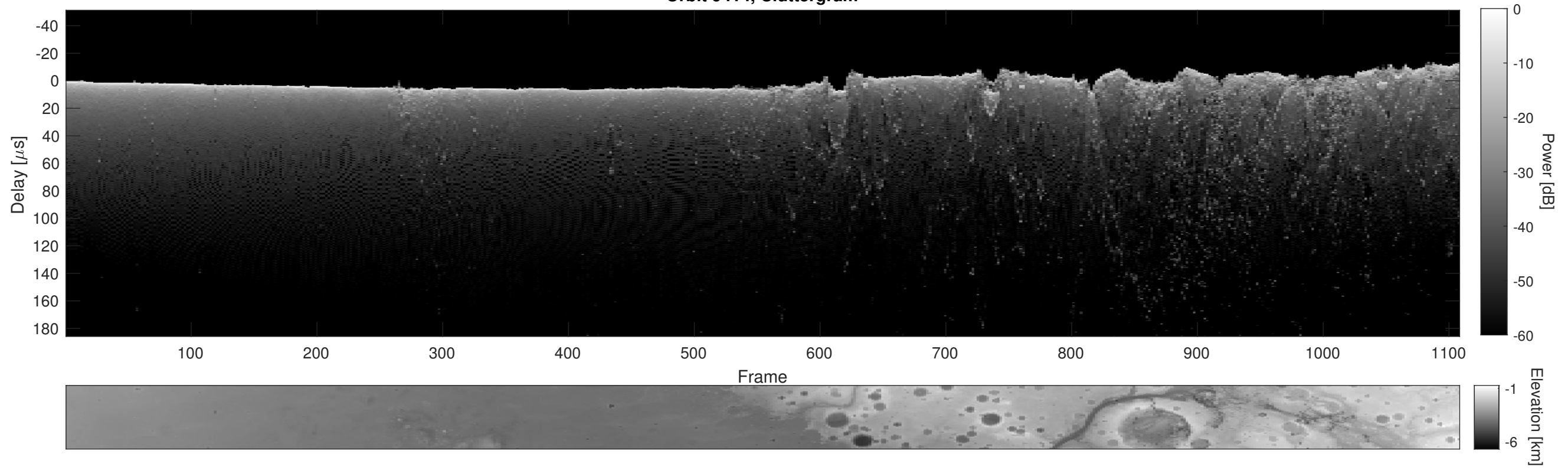
Orbit 9414, Cluttergram
