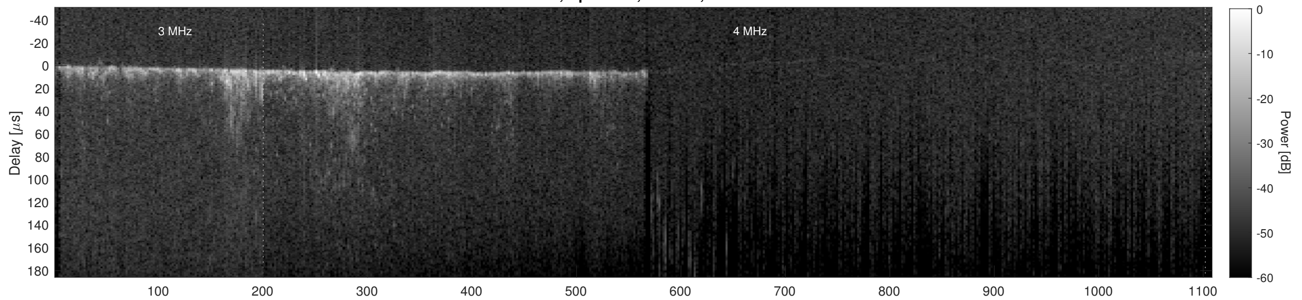
Orbit 9414, Cluttergram
